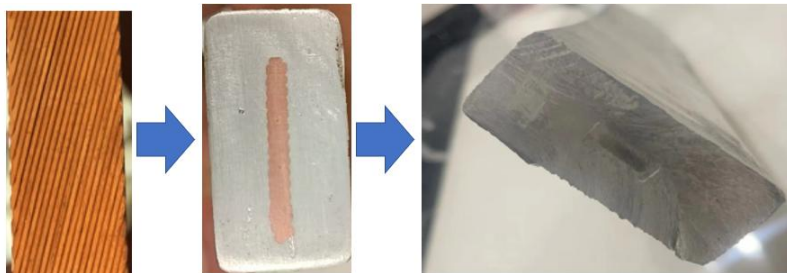
32 strands Rutherford cable First co-extrusion Second co-extrusion
