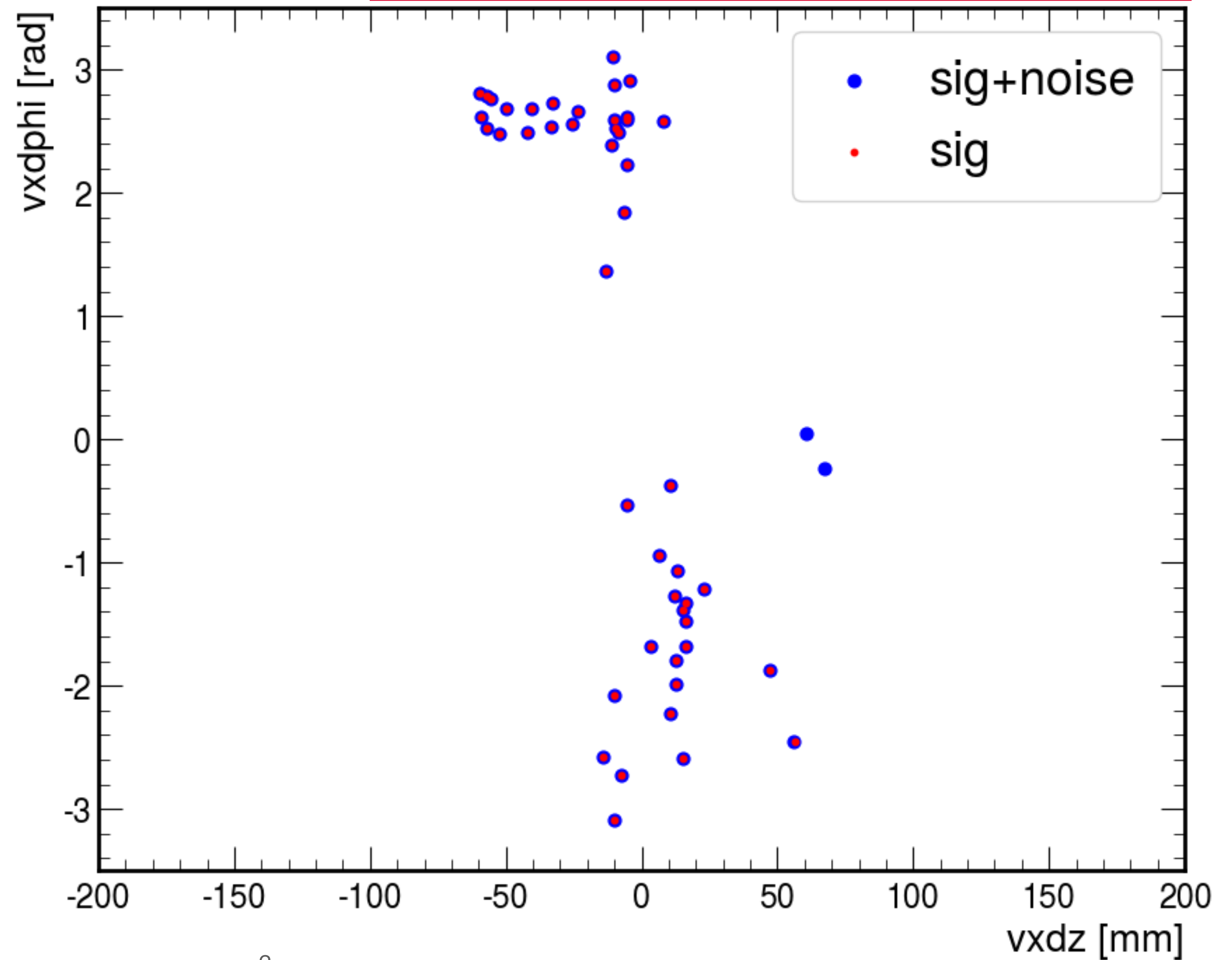
VXD L1 hits distribution of a ZH->mmbb event
