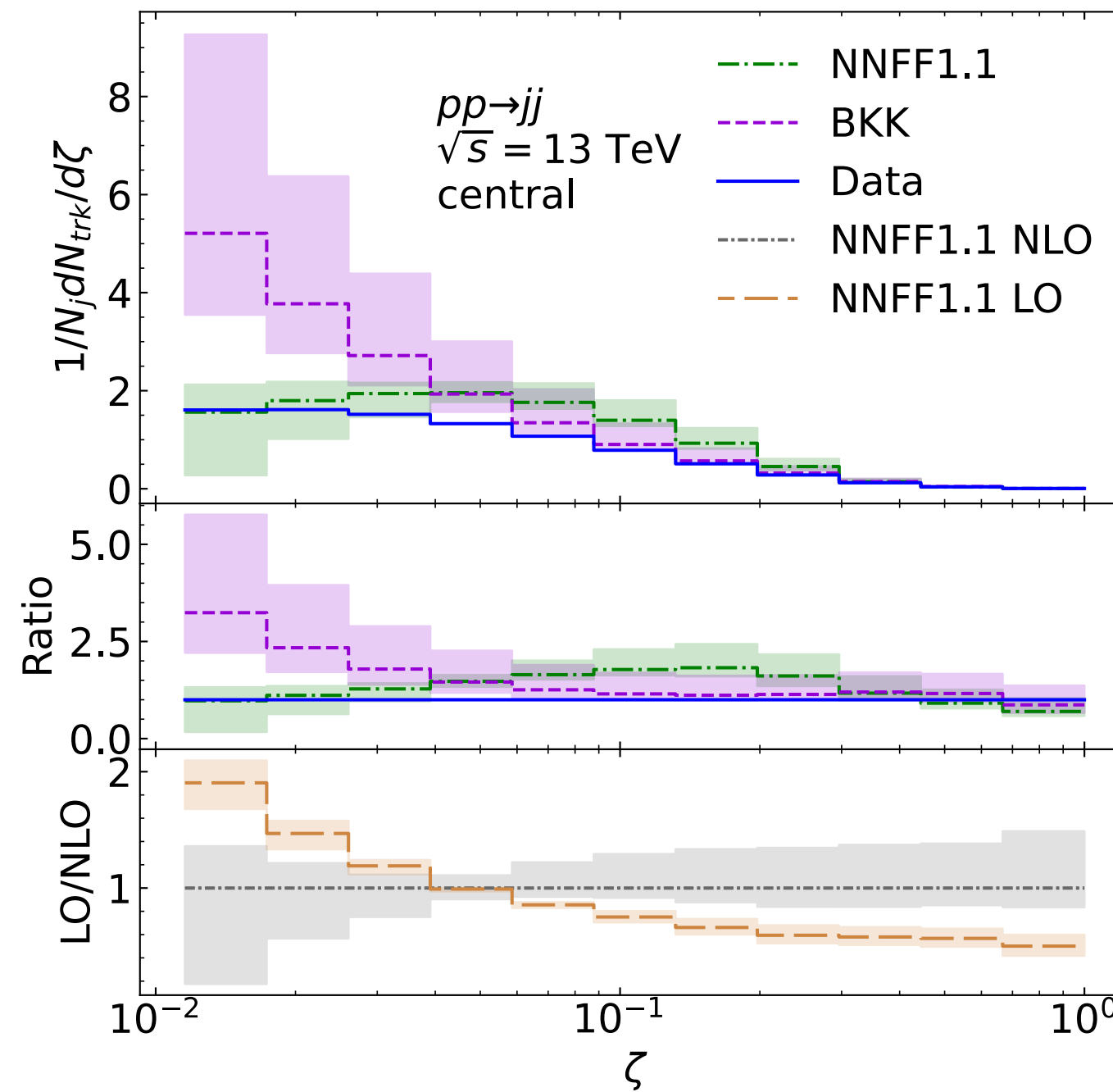
QCD inclusive dijets at LHC
