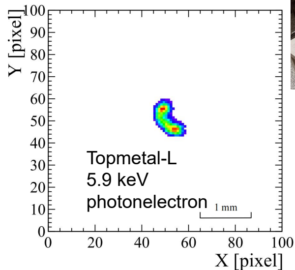
Topmetal-L
