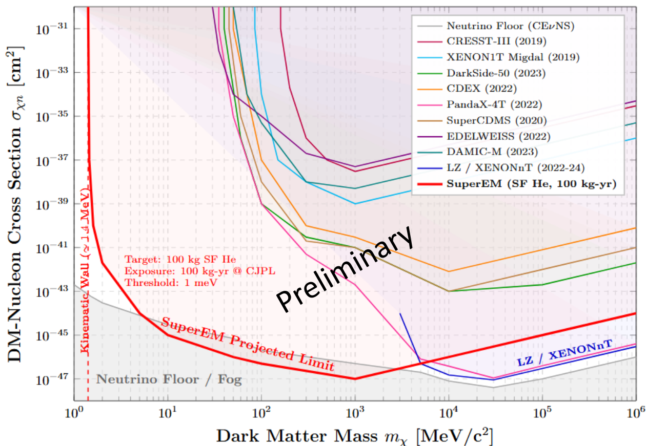
Projected LDM & WIMP Sensitivity: SuperEM with 100 kg SF He
