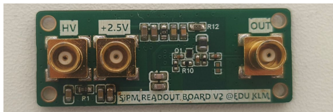
SiPM: MICROFJ-40035 (Sensl)
