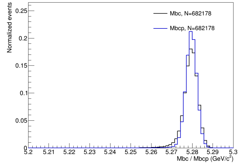
sigMC Mbc vs Mbc p comparison
