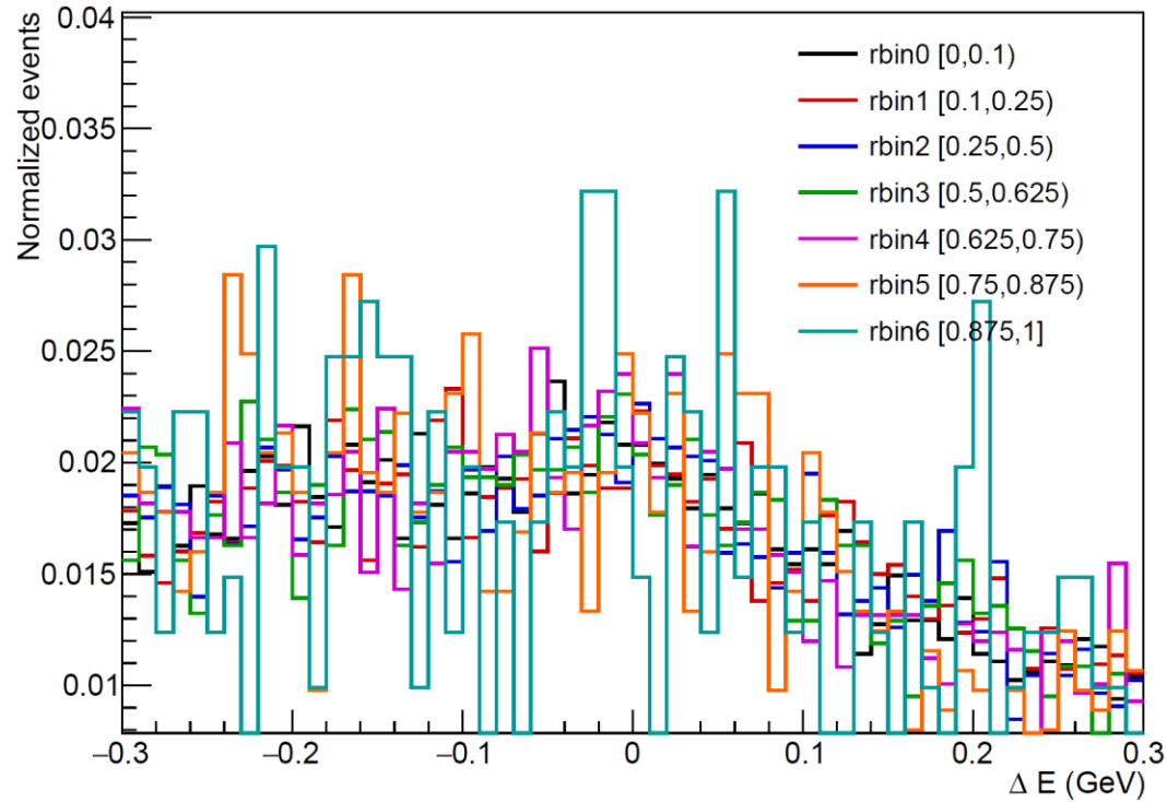
cont deltaE by r-bin
