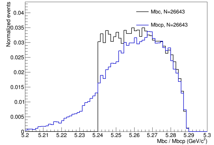
continuum Mbc vs Mbc p comparison
