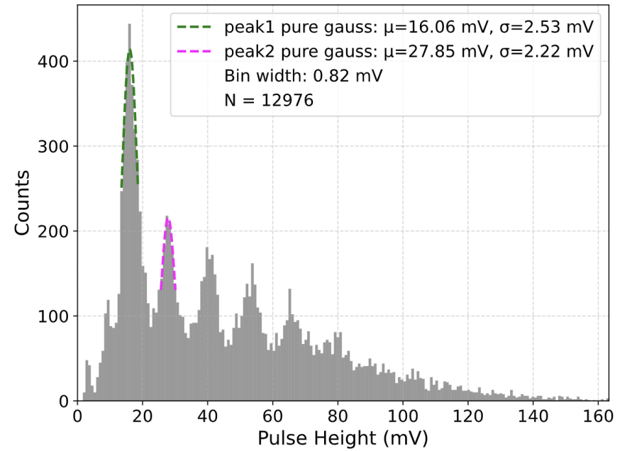
Channel: CH1 - Individual Pure Gauss Fits
