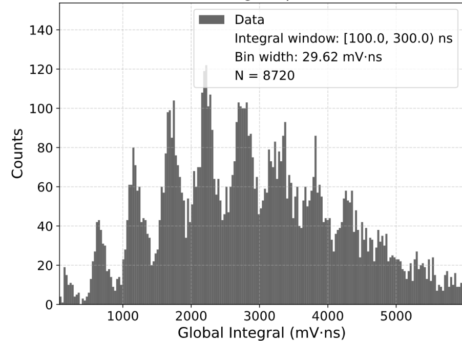
CH1 - Global Integral Spectrum (Clean)
