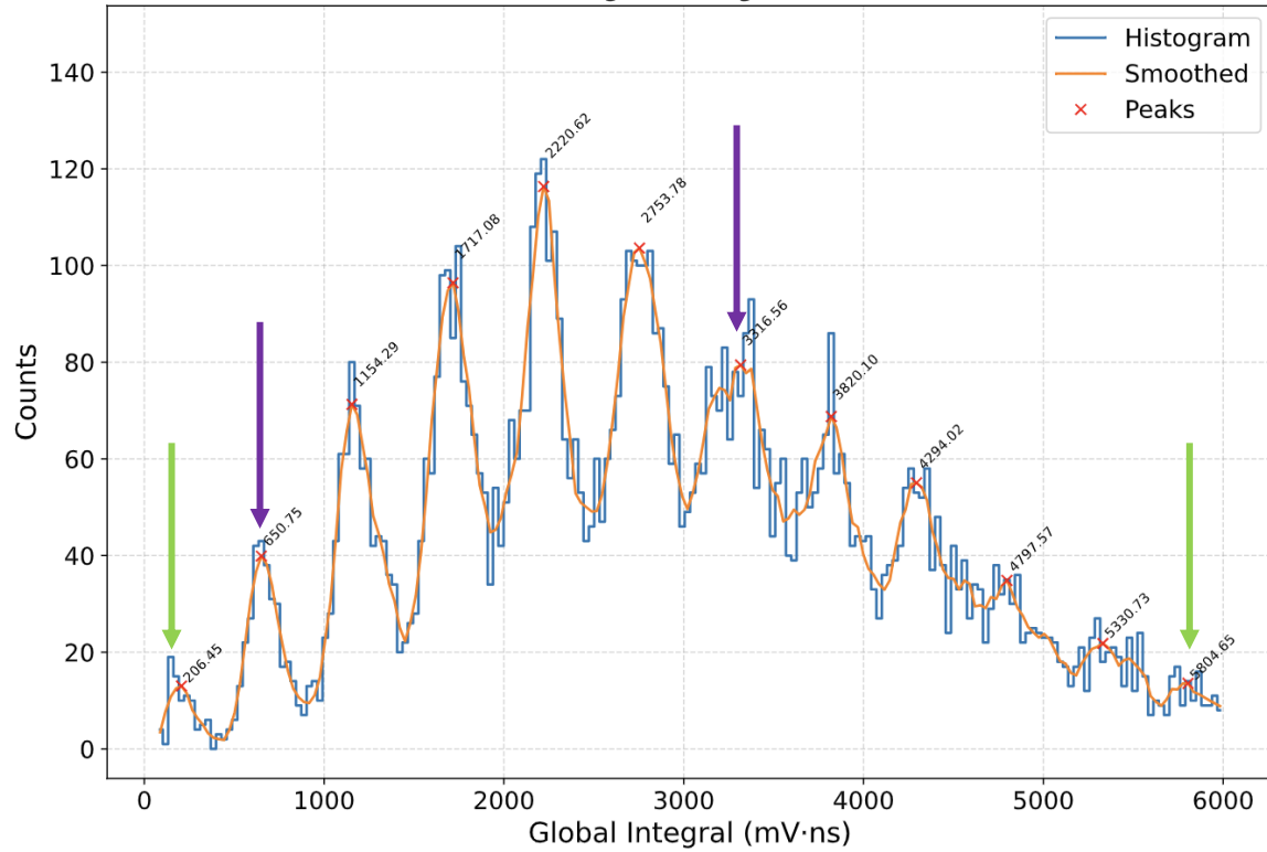
CH1 - Global Integral Histogram (8720 events)
