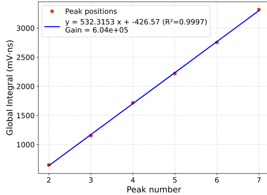
CH1 - Peak Position Linear Fit
