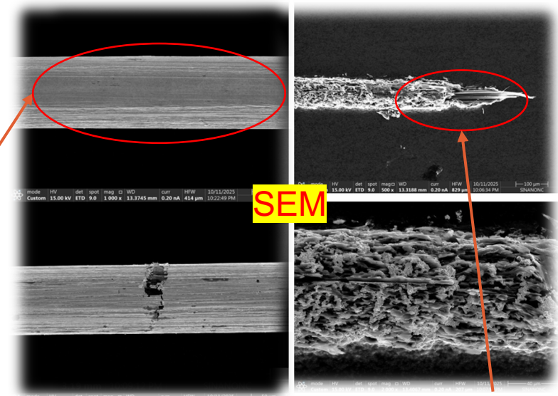
Fracture point
