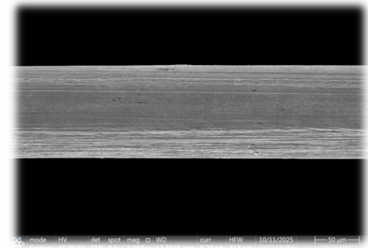
Tungsten-coated CNTF
