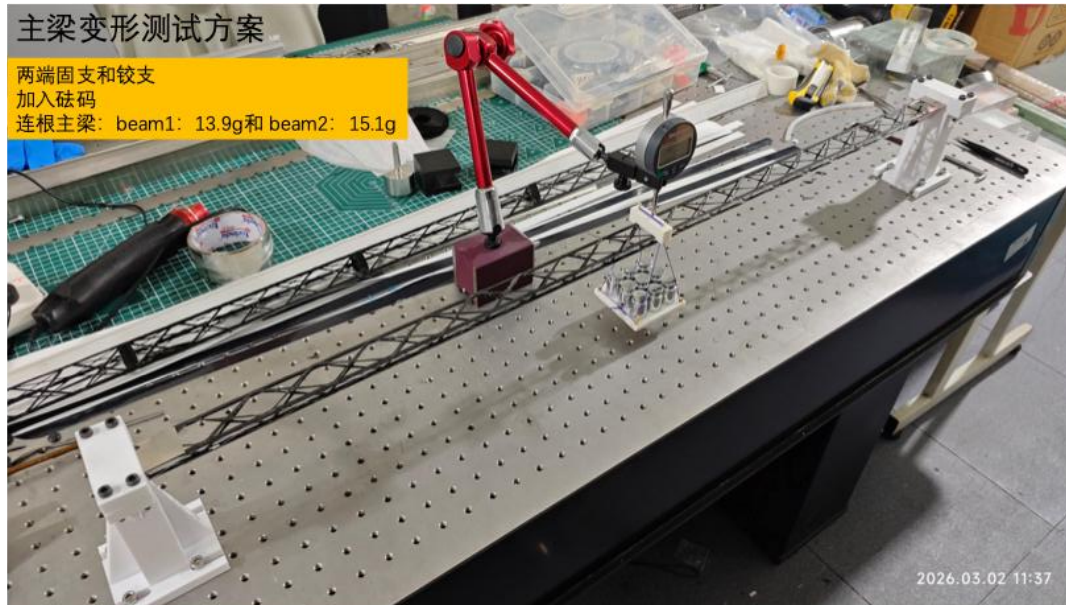
In-house 1m carbon-fiber structural prototype (mass: 15g): deformation under load
