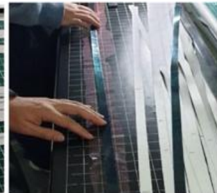
Laying up carbon-fiber prepreg
