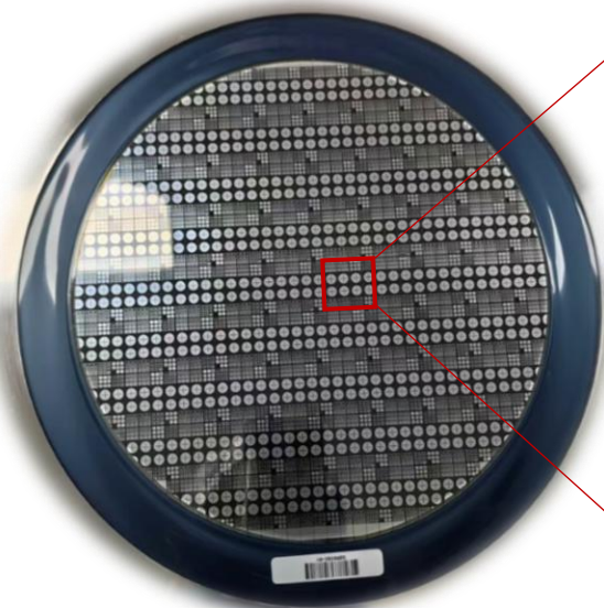
Latest SiC sensor wafer (3 rd iteration) 8-inch/MOSFET process line
