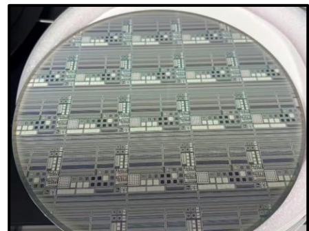
LGAD sensors wafer (2025)
