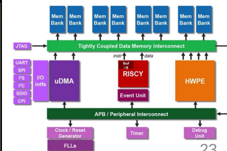
HERIS-V2 SoCCore architecture
