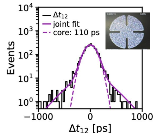
Test with 90 Sr β source timing resolution 77ps
