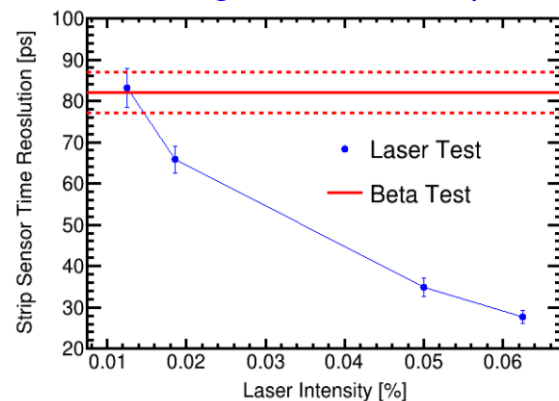
2cm strip sensor
