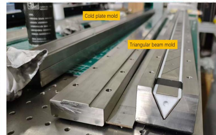
Custom-designed compression mold
