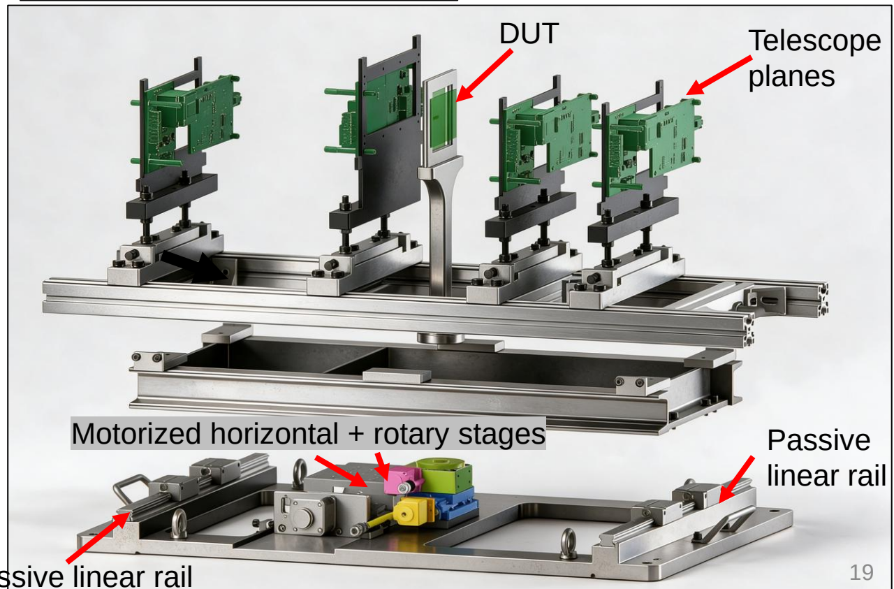
Telescope Design
