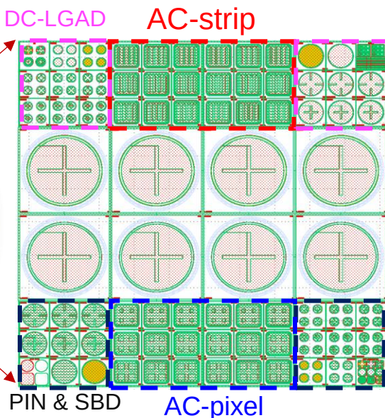
SiC sensor layout
