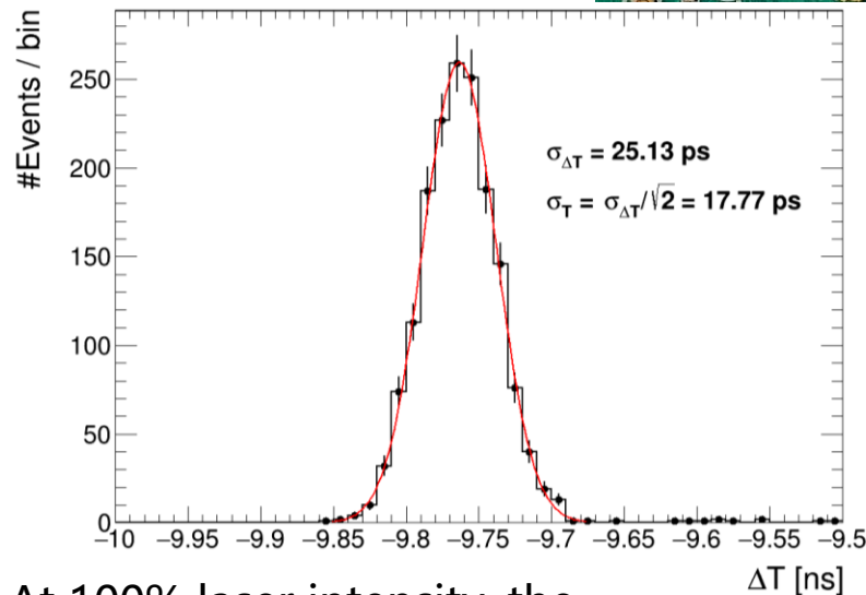
AC-LGAD pixel sensor (sensor size 2.5mm*2.5mm)
