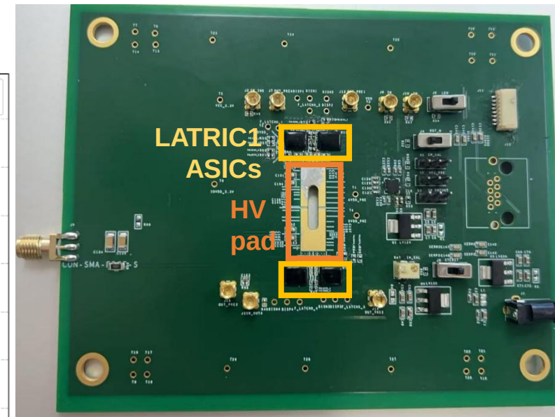
LATRIC1 & sensor test board
