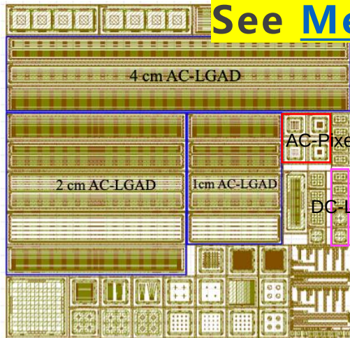
Sensor layout
