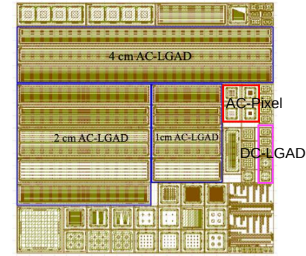
SiliconLGAD
