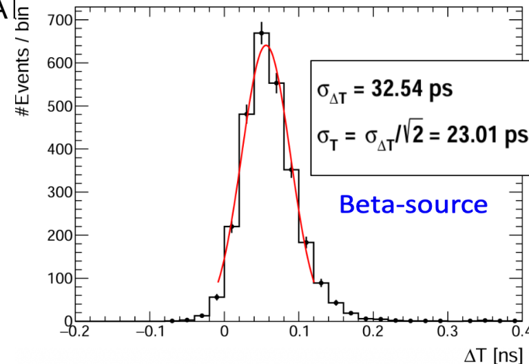
Time-difference distribution measured with two LATRIC1 ASICs
