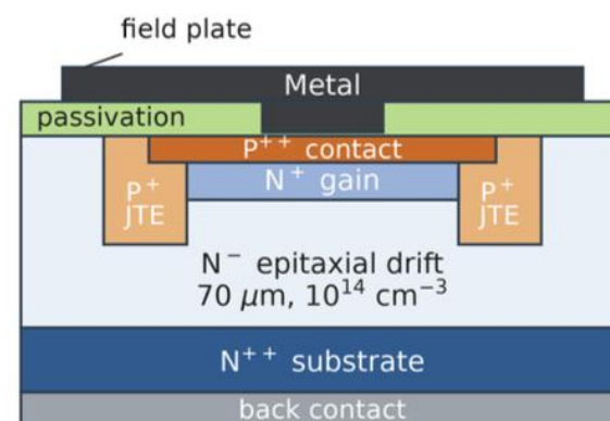
Implanted gain-type SiC (DC-gain) structure
