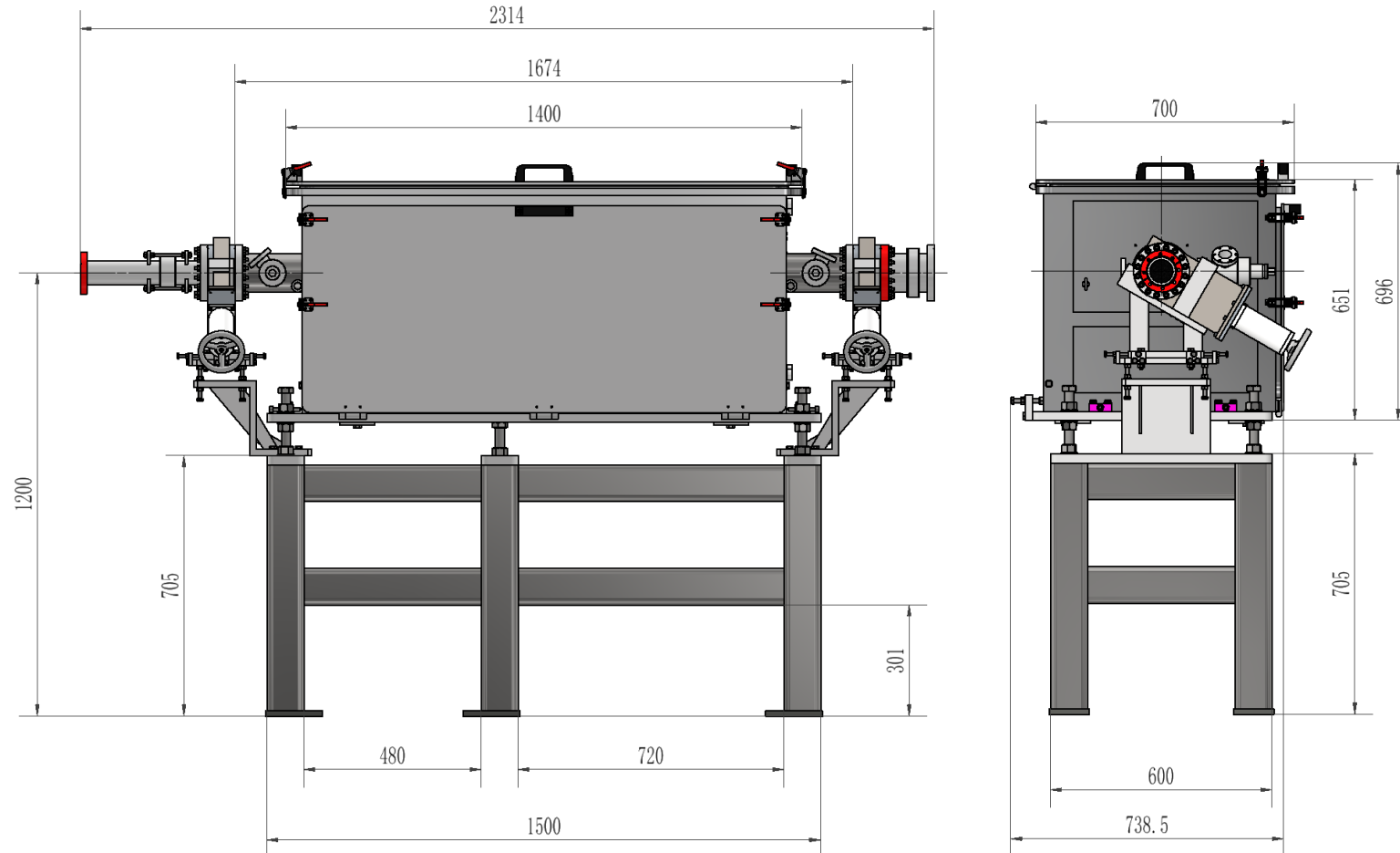
Mechanical design of the beam-test chamber
