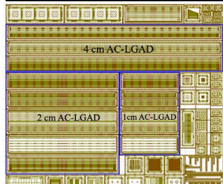
LGAD sensor layout (2025)
