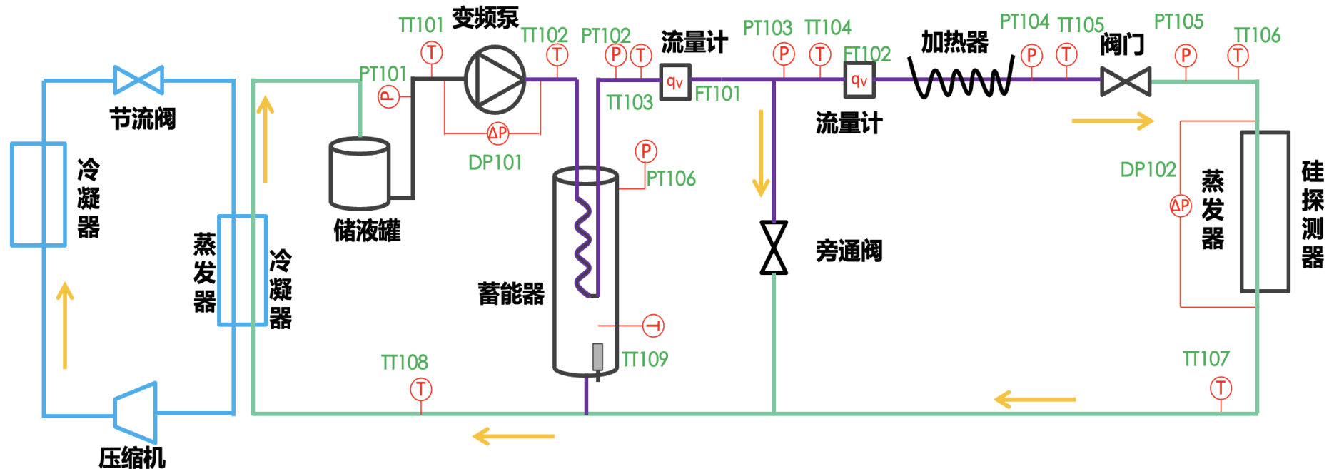
Two-phase CO 2 cooling system schematic
