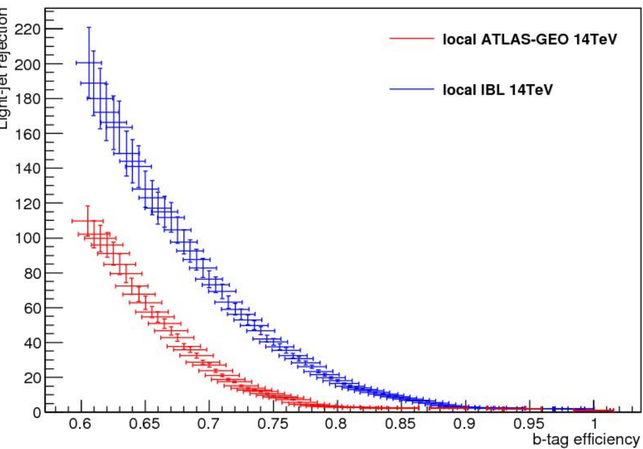
Efficiency v.s. Rejection with MV1
