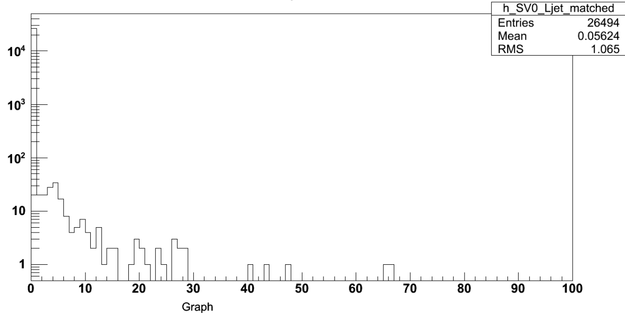
h_SV0_Ljet_matched
