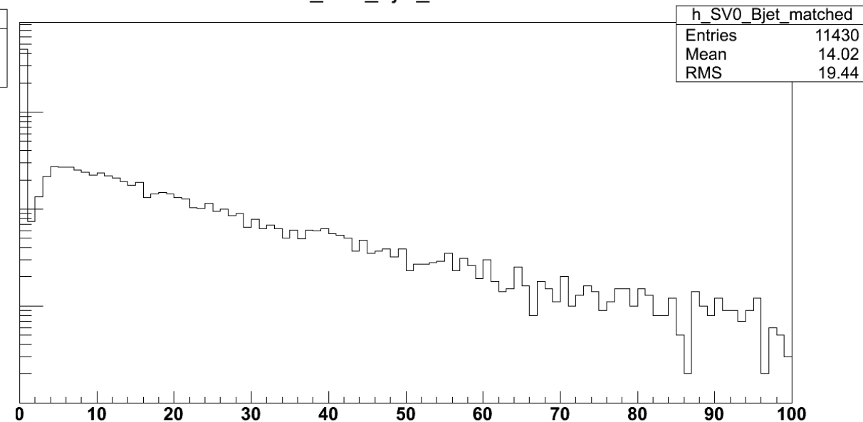
h_SV0_Bjet_matched
