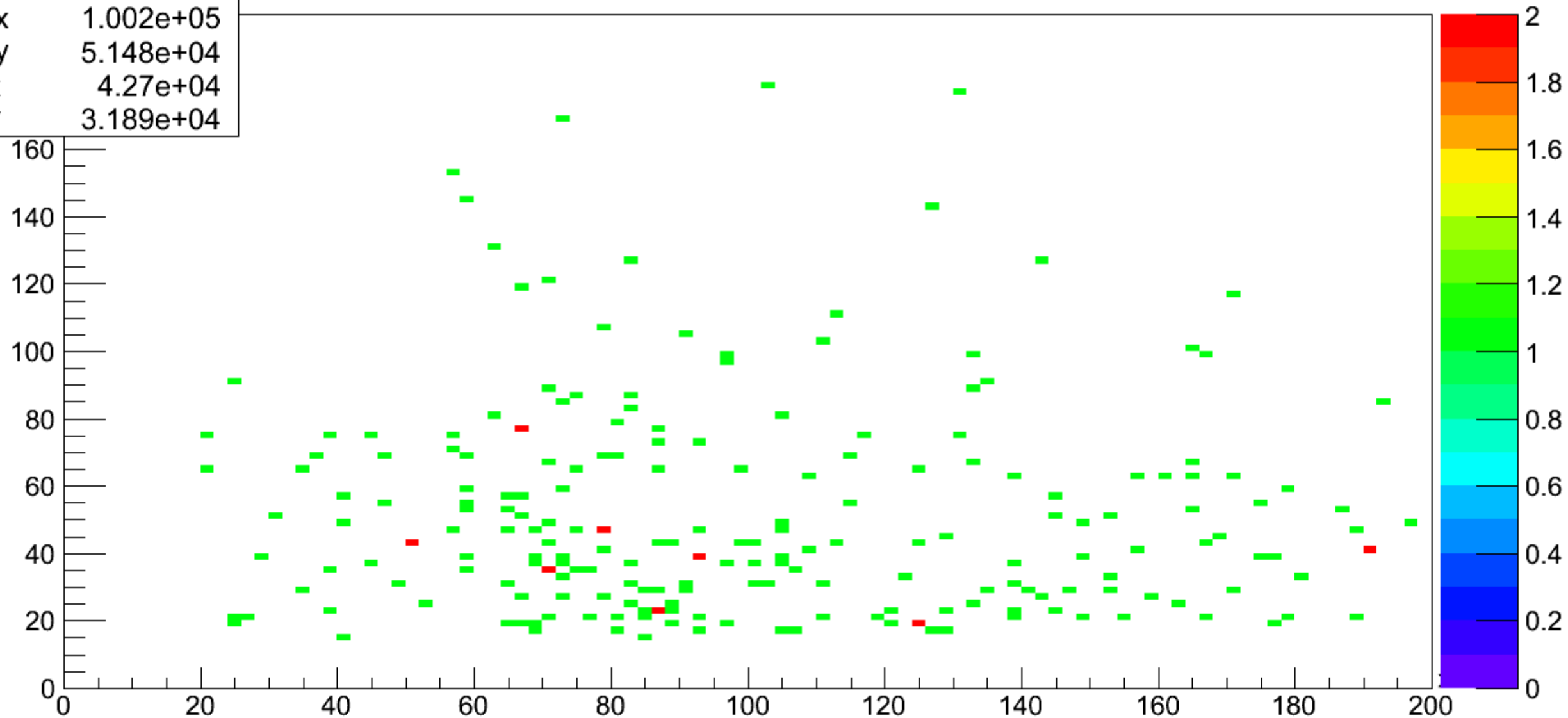
w hard mass vs w lep pt
