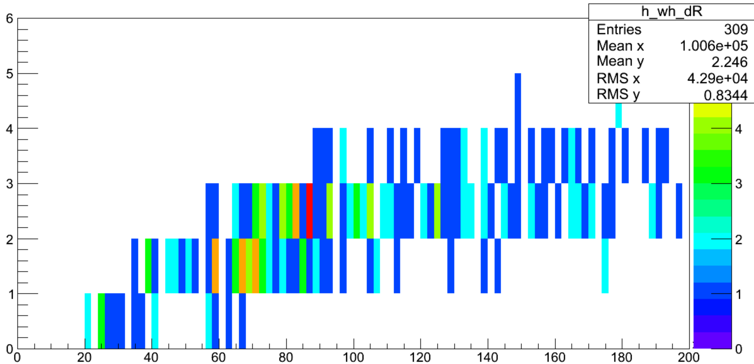
w hard mass vs dr JJ
