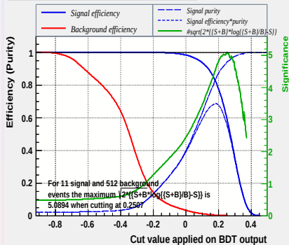
Cut efficiencies and optimal cut value
