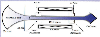
Basic klystron arrangement.
