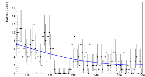
The efficiency \epsilon_{\gamma\gamma}^B with a + bx + cx^2 for continuous background extracted with 4-jets exclusive events
