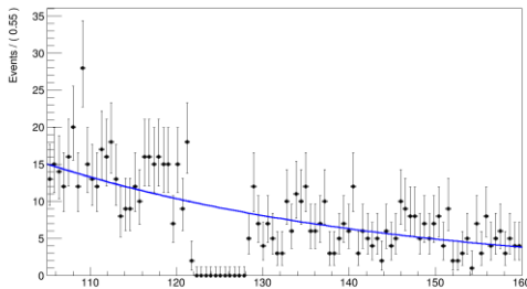
The efficiency \epsilon_{\gamma\gamma}^B with e^{ax} for continuous background extracted with 3-jets exclusive events
