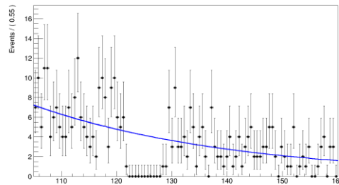
The efficiency \epsilon_{\gamma\gamma}^B with e^{ax} for continuous background extracted with 4-jets inclusive events
