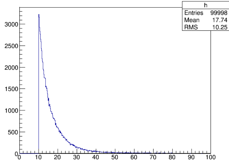
Hit Energy>10MeV
