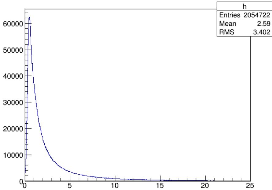
Hit Energy<10MeV
