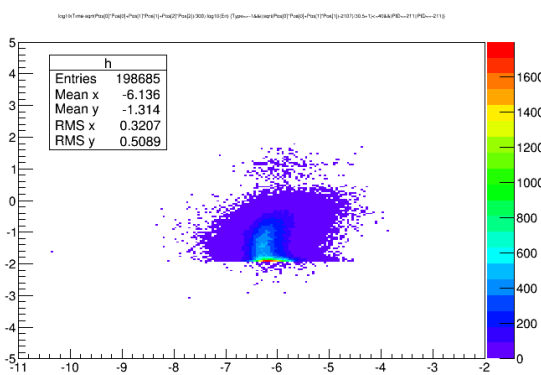
Pi 198685,17.9%
