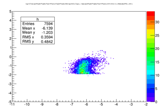
K, 7594, 0.7%
