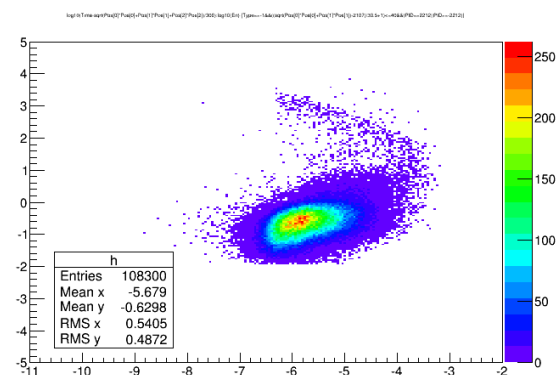
质子(108300,9.8%)
