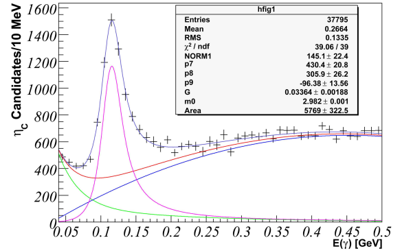
Fig. 1. Fit of CLEO data using d\Gamma/d\omega \sim \omega^3 \omega_0^2 / (\omega \omega_0 + (\omega - \omega_0)^2) BW(\omega) .
