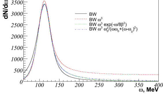
Fig. 6. Resulting signal line shapes for various d\Gamma/d\omega functions.
