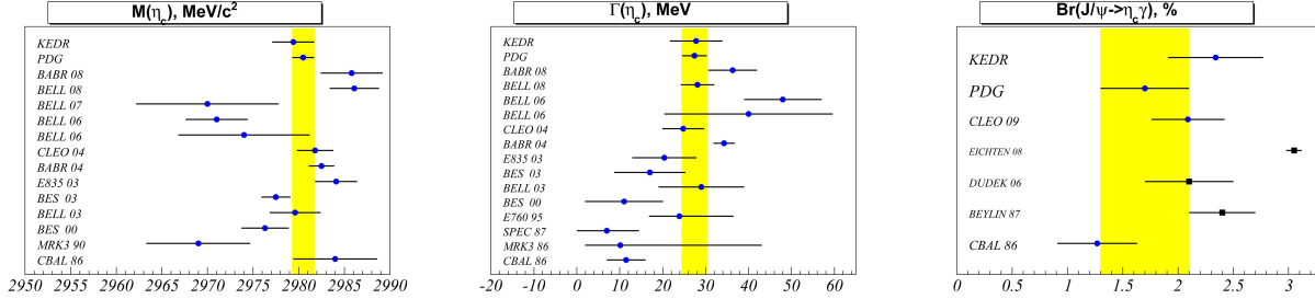
Fig. 7. \eta_c mass, width and \mathcal{B}(J/\psi \rightarrow \eta_c \gamma) measurements. The theoretical predictions for the branching fraction are also shown (squares).
