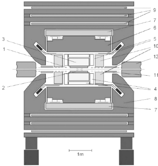
Fig. 3. KEDR detector. 1-vacuum chamber, 2-vertex detector, 3-drift chamber, 4-threshold aerogel counters, 5-ToF-counters, 6-liquid krypton calorimeter, 7-superconducting coil (0.65 T), 8-magnet yoke, 9-muon tubes, 10-CsI-calorimeter, 11-compensation solenoid, 12-VEPP-4M quadrupole.
