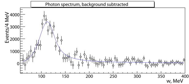
Fig. 5. Fit of the inclusive photon spectrum with f(\omega) = \omega_0^2 / (\omega\omega_0 + (\omega - \omega_0)^2) .
