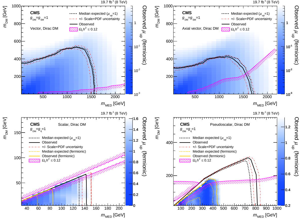
Figure 10: The 90% CL exclusion contours in the m_{\text{MED}} - m_{\text{DM}} plane assuming vector (top-left), axial vector (top-right), scalar (bottom-left), and pseudoscalar (bottom-right) mediators. The scale shown on the right hand axis shows the expected 90% CL exclusion upper limit on the signal strength, assuming the mediator only couples to fermions. For the scalar and pseudoscalar mediators, the exclusion contour assuming coupling only to fermions (fermionic) is also shown. The white region shows model points that were not tested when assuming coupling only to fermions and are not expected to be excluded by this analysis under this assumption. The red dot-dashed lines indicate the variation in the exclusion contours due to modifying the renormalization and factorization scales by a factor of two in the generation of the signal. In all cases, the excluded region is to the bottom-left of the contours, except for the relic density, which shows the regions for which \Omega_c h^2 = 0.12 , as indicated by the shading. In all of the models, the mediator width is determined using the minimum width assumption.
