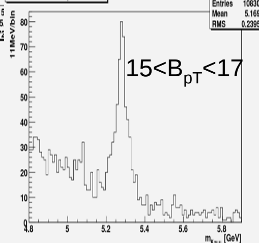
Inv. mass of J/\psi and K\pi
