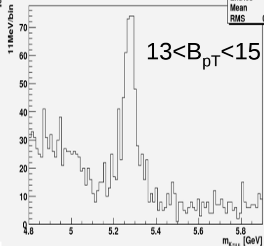
Inv. mass of J/\psi and K\pi
