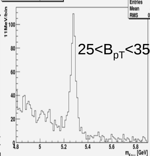
Inv. mass of J/\psi and K\pi
