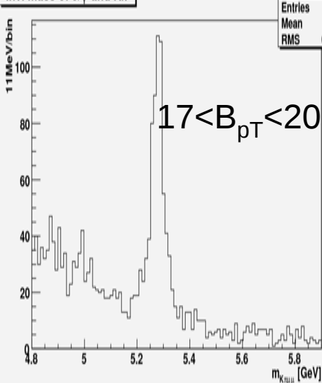
Inv. mass of J/\psi and K\pi
