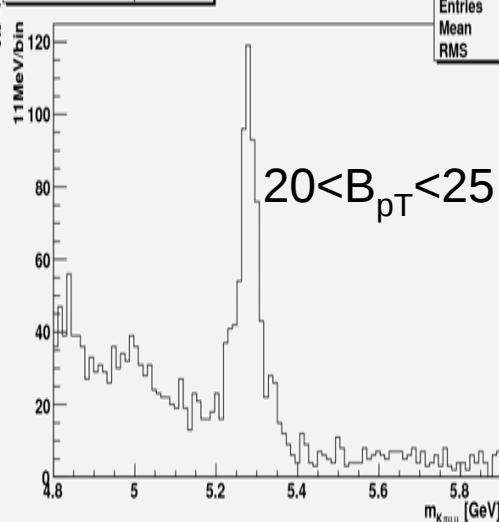
Inv. mass of J/\psi and K\pi
