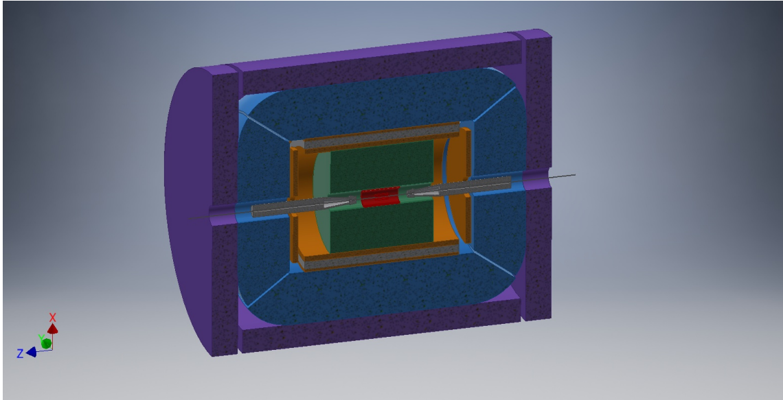
Figure 3.11: Schematic layout of the IDEA detector. Sub-detectors are outlined in different colors : vertex detector (red), drift chamber (green), pre-shower (orange), magnet (gray), calorimeter (blue), magnet yoke and muon system (violet).
