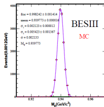
(h) Recoiling mass of \Lambda\pi^0
