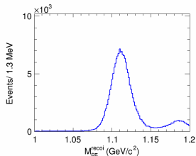
(f) Recoiling mass of p\pi
