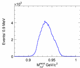
(g) Recoiling mass of p\pi\pi^0
