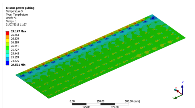
Figure 5.27: Temperature distribution in an active layer of the SDHCAL operated with no power-pulsing. The cooling system is made of a circulating water inside copper tubes in contact with the ASICs.
