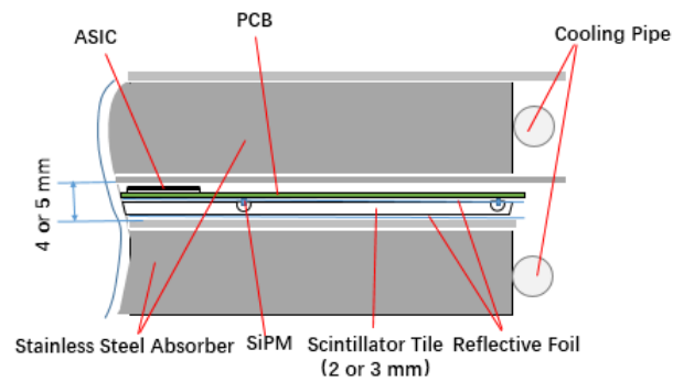
Figure 5.38: Side view of one layer in AHCAL
