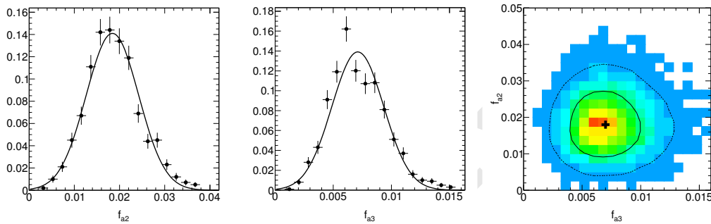
Figure 11.17: Distribution of fitted values of f_{a2} and f_{a3} in a large number of generated experiments. In the left and middle plots, only the parameter shown is floated. Other parameters are fixed to SM expectations. Right plot: simultaneous fit of non-zero f_{a2} and f_{a3} , with 68% and 95% confidence level contours shown. Keep the right plot only?
