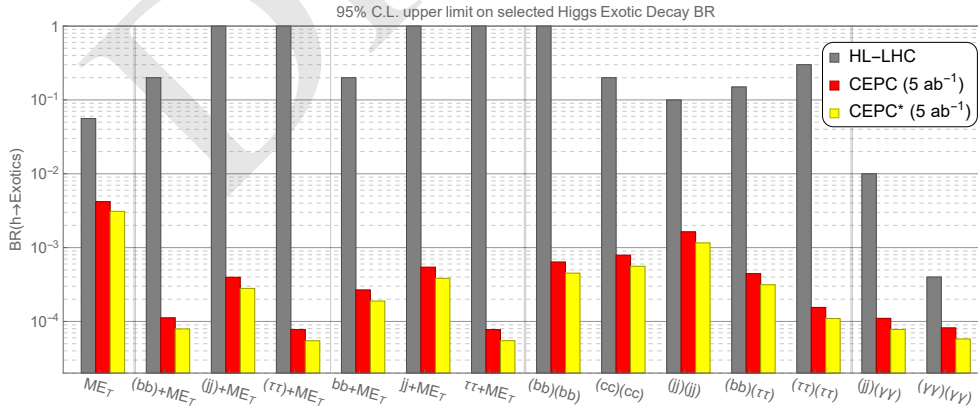
Figure 11.16: The 95% C.L. upper limit on selected Higgs boson exotic decay branching fractions at HL-LHC and CEPC, based on Ref [74]. The benchmark parameter choices are the same as in Table 11.9. The red bars correspond to the results using leptonically decaying spectator Z-boson alone. The yellow bars further include extrapolation with the inclusion of the hadronically decaying Z-bosons. Several vertical lines are drawn in this figure to divide different types of Higgs boson exotic decays.
