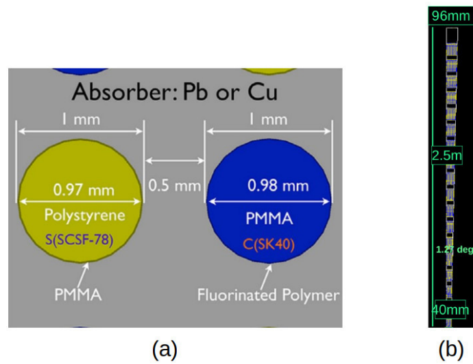
Figure 5.47: (a) Fibre arrangement inside the modules. (b) Dimensions of a module in the barrel region (at \eta = 0 ): from inside to outside the number of fibres more than doubles.
