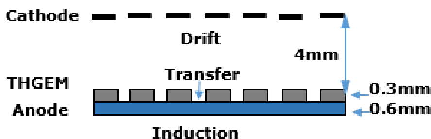
Figure 5.31: The schematic diagram of the WELL-THGEM.
