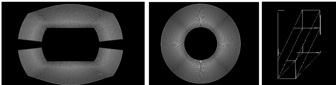
Figure 5.48: An alternative 4\pi solution (called "wing" geometry).
