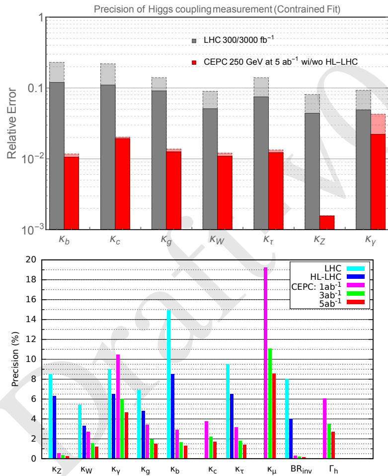
Figure 12.1: Top: The 7 parameter fit, and comparison with the HL-LHC, discussed in detail in Chapter 10. The projections for CEPC at 250 GeV with 5 \text{ab}^{-1} integrated luminosity are shown. The CEPC results without combination with HL-LHC input are shown with dashed edges. The LHC projections for an integrated luminosity of 300 \text{fb}^{-1} are shown in dashed edges. Bottom: Comparison between the LHC and several benchmark luminosities of the CEPC.
