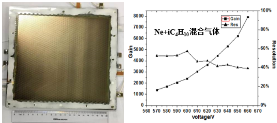
Figure 5.32: The photograph(left) and performance (right) of the WELL-THGEM detector.
