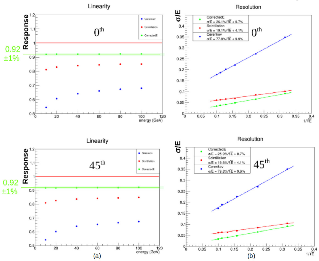
Figure 5.61: Linearity and energy resolution with pions, for towers #0 (top) and #45 (bottom), in the wedge geometry.
