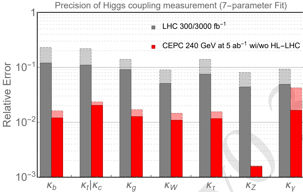
Figure 11.9: The 7 parameter fit result, and comparison with the HL-LHC [23]. The projections for the CEPC at 240 GeV with 5 ab^{-1} integrated luminosity are shown. The CEPC results without combination with the HL-LHC input are shown with dashed edges. The LHC projections for an integrated luminosity of 300 fb^{-1} are shown in dashed edges.
