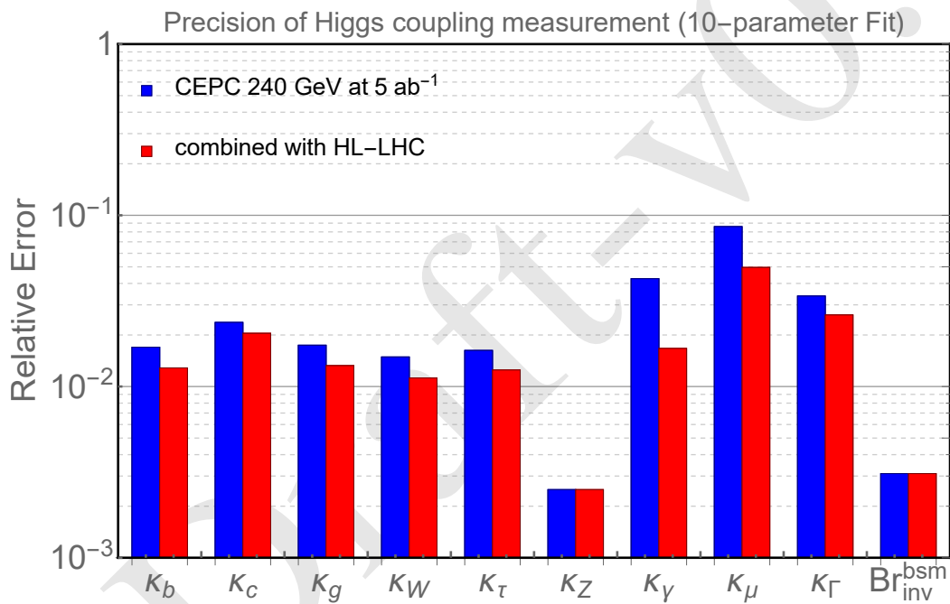
Figure 11.10: The 10 parameter fit result for CEPC at 240 GeV with 5 ab -1 integrated luminosity (blue) and in combination with HL-LHC inputs (red). All the numbers refer to are relative precision except for BR_{inv}^{bsm} for which 95% CL upper limit are quoted respectively.
