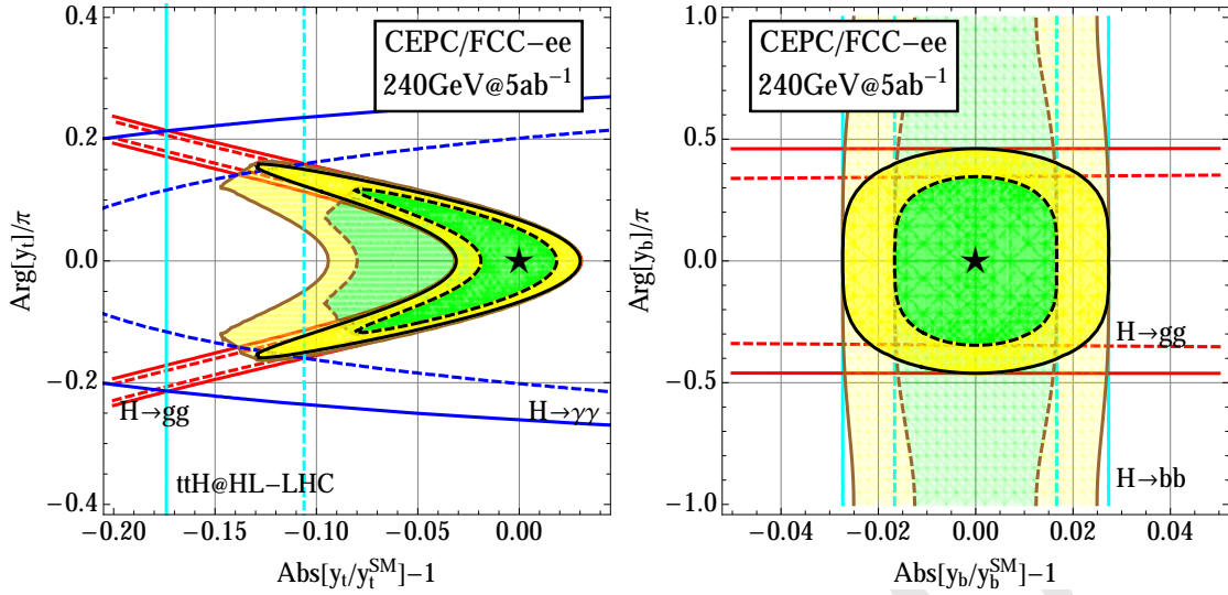
Figure 11.14: Results for analysis on C_{y_t} and C_{y_b} in the projected allowed regions for modification to top and bottom Yukawa couplings in magnitude and CP phase at 68% and 95% confidence level. The combined results for CEPC are shown in black curves. The source of individual constraints for the single operator analysis are labeled correspondingly. For a joint analysis of simultaneous appearance of both \mathcal{O}_{y_t} and \mathcal{O}_{y_b} operators, the results for CEPC are shown in the enlarged yellow (95%) and green regions (68%) with thick brown boundary lines.
