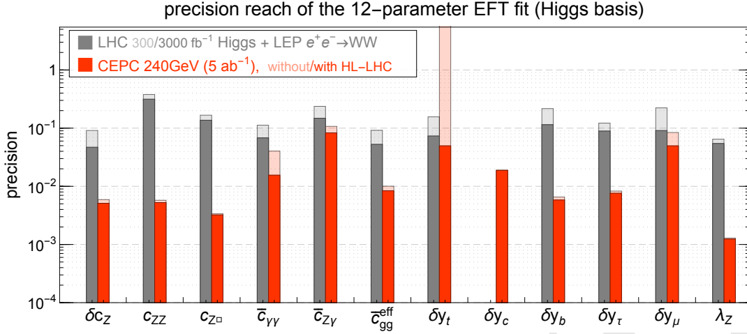
Figure 11.11: One-sigma precision reach of the twelve parameters in the Higgs basis. The first column shows the results from the LHC Higgs measurements with 300 \text{ fb}^{-1} (light shade) and 3000 \text{ fb}^{-1} (solid shade) combined with LEP diboson ( e^+e^- \rightarrow WW ) measurement. The second column shows the results from CEPC with 5 \text{ ab}^{-1} data collected at 240 GeV with unpolarized beam. The results from CEPC alone are shown in light shades, and the ones from a combination of CEPC and HL-LHC are shown in solid shades. \delta y_c is fixed to zero for the LHC fits.
