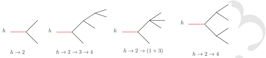
Figure 11.15: The topologies of the SM-like Higgs boson exotic decays.
