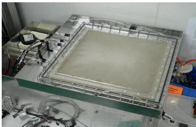
Figure 5.30: The maximum size of THGEM produced in domestic currently ( 40 \times 40 \text{ cm}^2 ).
