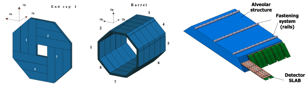
Figure 5.3: Left: Geometry of the SiW-ECAL Endcaps. Middle: Barrel Right: Geometry of the barrel modules.
