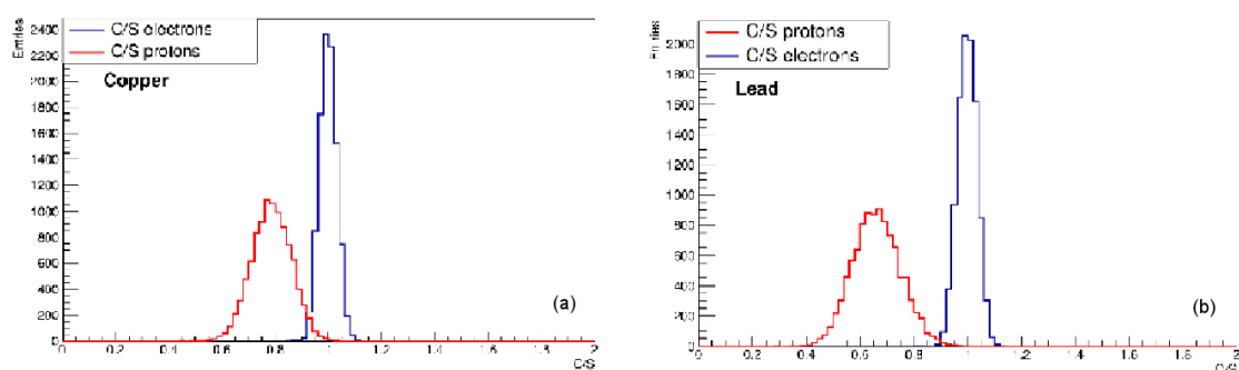
Figure 5.58: C/S ratio for 80 GeV e^- and protons in copper (a) and lead (b).
