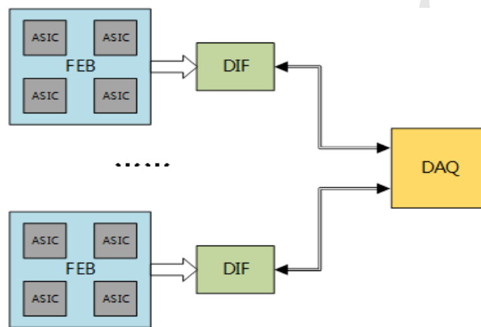
Figure 5.33: The schematic diagram of the readout system.
