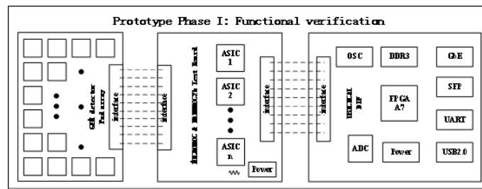
Figure 5.34: The diagram of the phase I design.
