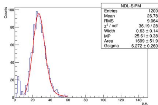
Figure 5.44: Sr-90 electron source test result of scintillator detector cell readout by NDL-SiPM
