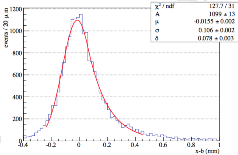
Figure 4.35: Measured drift distance residue distribution in the MEG2 drift chamber prototype under cosmic rays, indicating a resolution of less than 110 \mu m , averaged over all drift times and in a wide range of track angles. 85\% He - 15\% iC_4H_{10} gas mixture.
