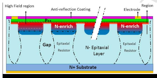
Figure 5.43: Schematic structure of EQR SiPM; APD cell consists of N-enriched regions forming high electric fields between the N-type epitaxial silicon wafer and the P++ surface layer, the un-depleted region in the epitaxial silicon layer below the P/N junction as the quenching resistor, and the APD cells are isolated from each other by the Gap depletion region.
