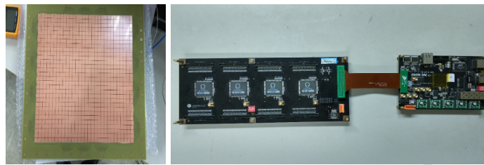
Figure 5.35: Pictures for the phase I design.
