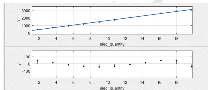
Figure 5.16: Pedestal noise.
