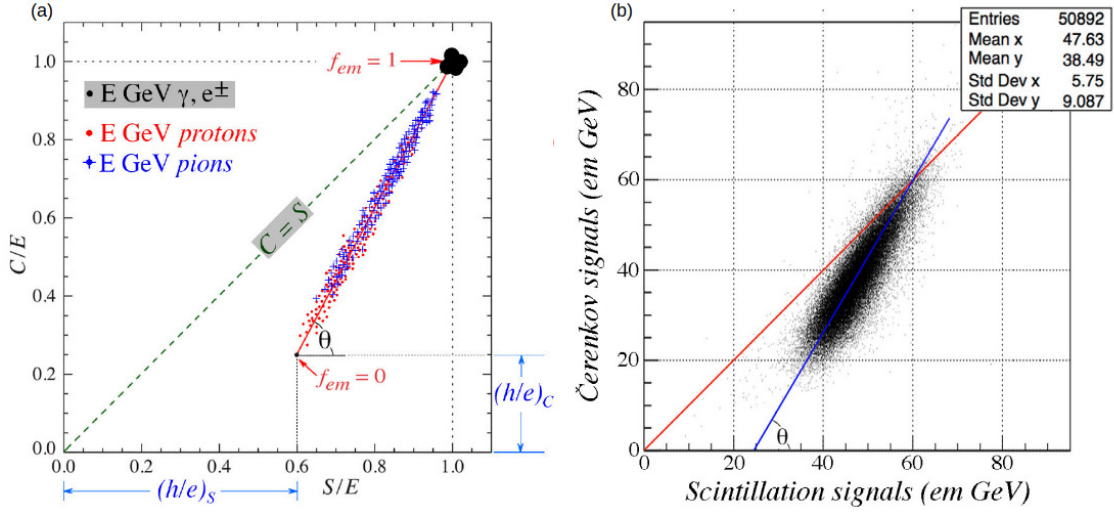
Figure 5.45: (a) Scatter plot of C/E versus S/E in a dual-readout calorimeter for p and \pi ; (b) scatter plot of C and S signals for 60 GeV pions in the RD52 dual-readout lead-fibre calorimeter.
