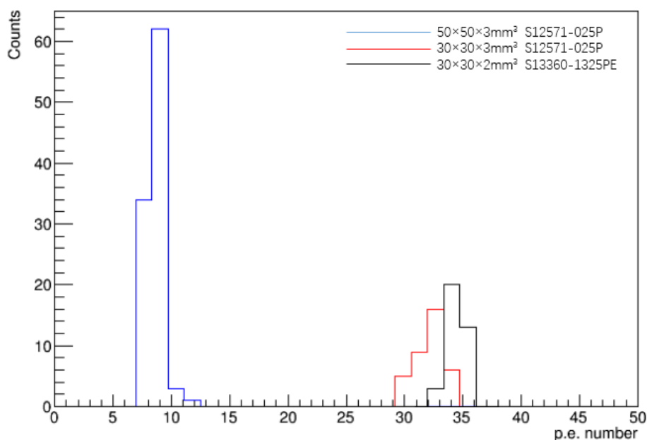
Figure 5.42: The uniformity measurement result of 30 \times 30 \times 3 \text{mm}^3 , 50 \times 50 \times 3 \text{mm}^3 and 30 \times 30 \times 2 \text{mm}^3 detector cell
