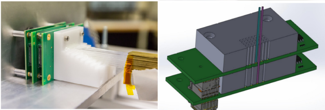
Figure 5.50: Staggered readout scheme: the scintillation and Čerenkov fibres are readout at different planes to avoid light leakage into neighbouring channels.
