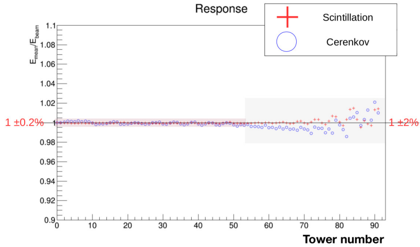
Figure 5.59: Ratio of reconstructed energy to the beam energy for 20 GeV e^- , as a function of the tower number, in the wedge geometry.
