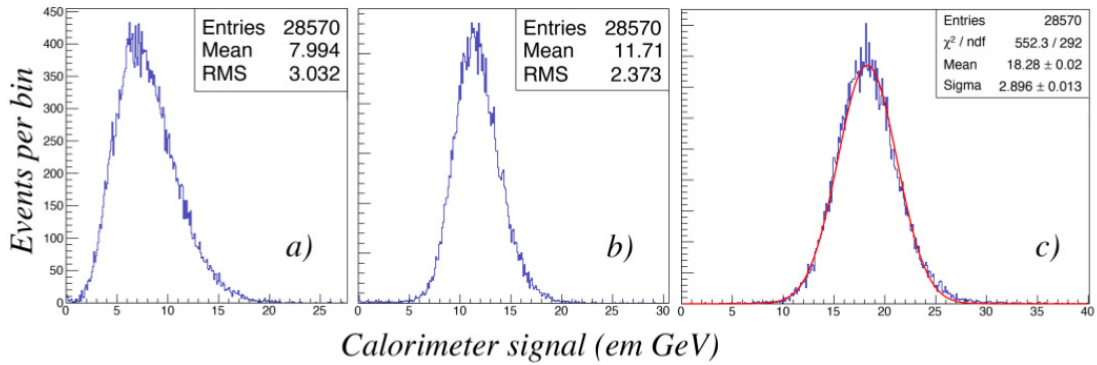
Figure 5.53: Signal distributions for 20 GeV \pi^- particles in a lead-fibre matrix. Shown are the measured (a) Čerenkov and (b) scintillation signal distributions as well as (c) the distribution obtained by combining the two signals according to Equation 5.8, with \chi = 0.45 .
