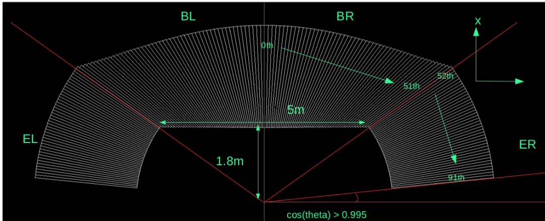
Figure 5.46: A possible 4\pi solution (called "wedge" geometry).
