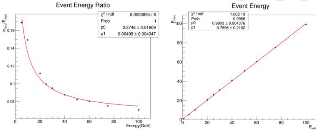
Figure 5.41: Left figure is energy resolution, right figure is the result of reconstruction energy linearity
