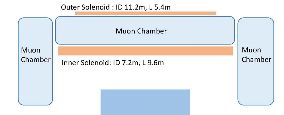
Figure 6.5: The sketch of dual solenoid design
