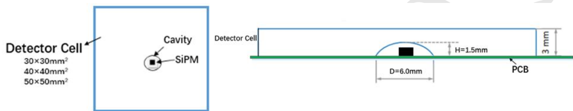
Figure 5.39: Top view of a detector cell (left) and sectional view of a detector cell with a dome-shaped cavity (right)
