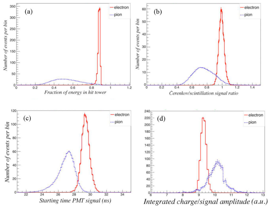
Figure 5.54: Distribution of four discriminating variables for 60 or 80 GeV electrons and pions: (a) energy fraction deposited in the hit tower; (b) C/S signal ratio in the hit tower; (c) starting time of the PM signal; (d) ratio of the integrated charge and the amplitude of the signals.
