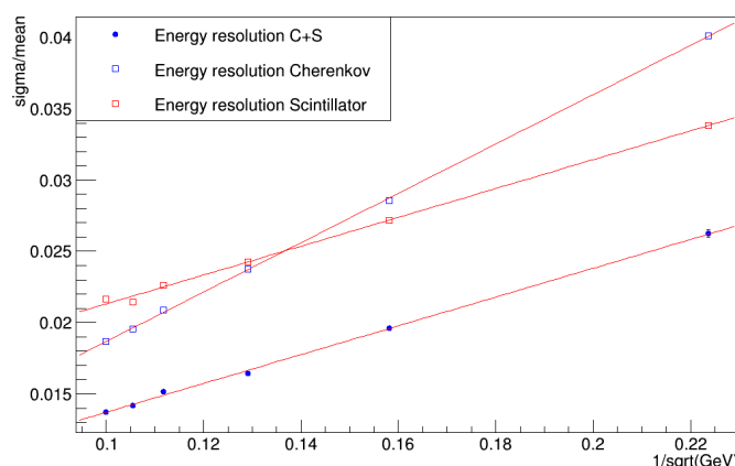
Figure 5.56: Relative resolution for em showers for the C and S signals, independently, and for the average of the two.
