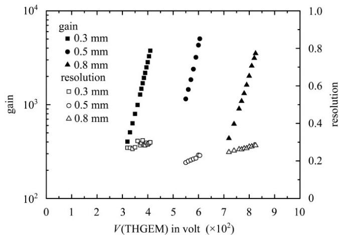
Figure 5.29: Gain and energy resolution of THGEM detector obtained with 55 Fe.
