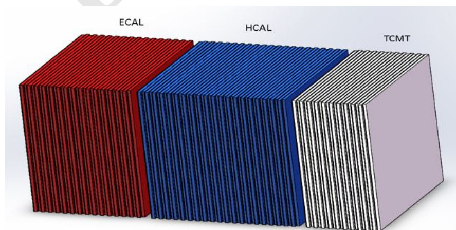
Figure 5.40: The structure of simulated calorimeters which is a part of the simplify geometry. Red part is the the Silicon ECAL, Blue part is the scintillator AHCAL
