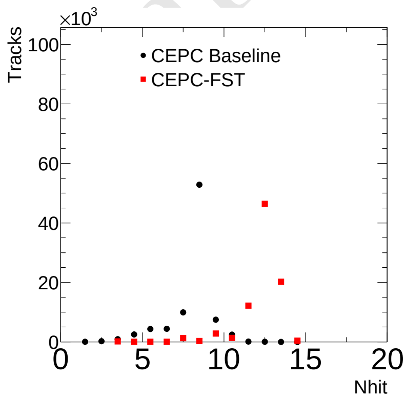
Figure 4.31: The distributions are shown for the number of silicon hits on the track.
