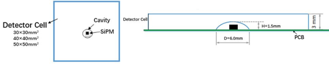
Figure 5.23: Top view of a detector cell (left) and cross sectional view of a detector cell with a dome-shaped cavity (right)
