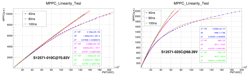
Figure 5.4: The response curve of 10000-pixel(left) and 1600-pixel(right) SiPMs for different illuminating durations.
