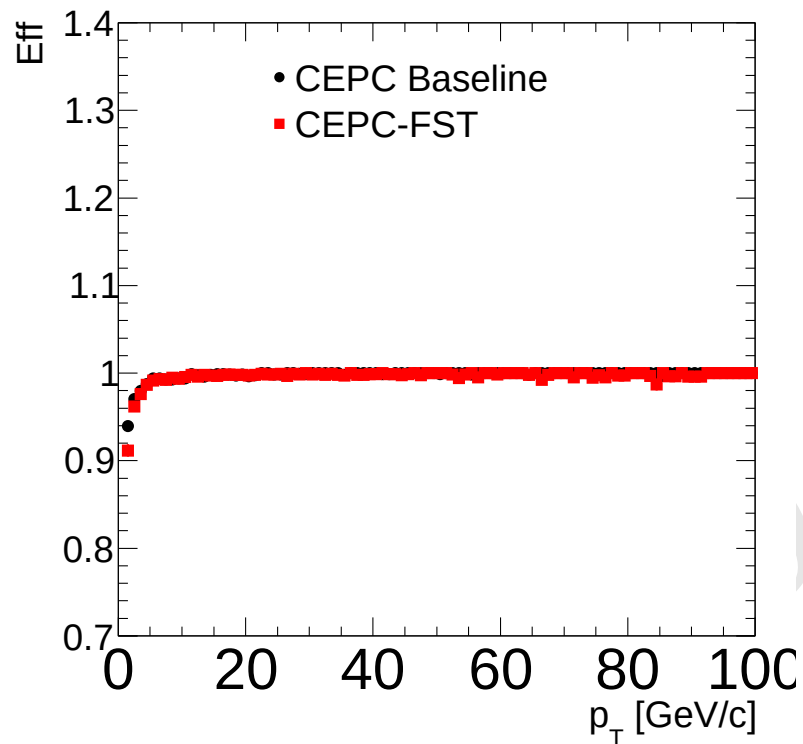
Figure 4.30: The tracking efficiencies are measured as function of p_T for single muons using CEPC baseline (v_4) and CEPC-FST detetcors.
