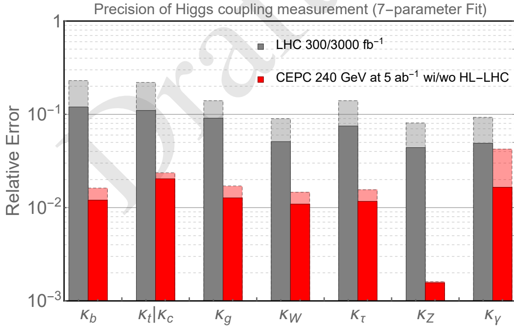
Figure 11.8: The 7 parameter fit result, and comparison with the HL-LHC [23]. The projections for the CEPC at 240 GeV with 5 \text{ab}^{-1} integrated luminosity are shown. The CEPC results without combination with the HL-LHC input are shown with dashed edges. The LHC projections for an integrated luminosity of 300 \text{fb}^{-1} are shown in dashed edges.
