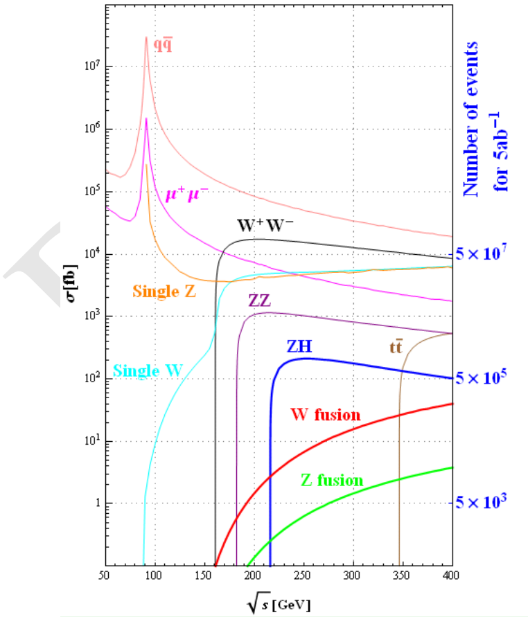
Figure 3.1: Cross sections of the leading Standard Model processes at non polarized electron positron collision (Left) and at proton collision (Right)
