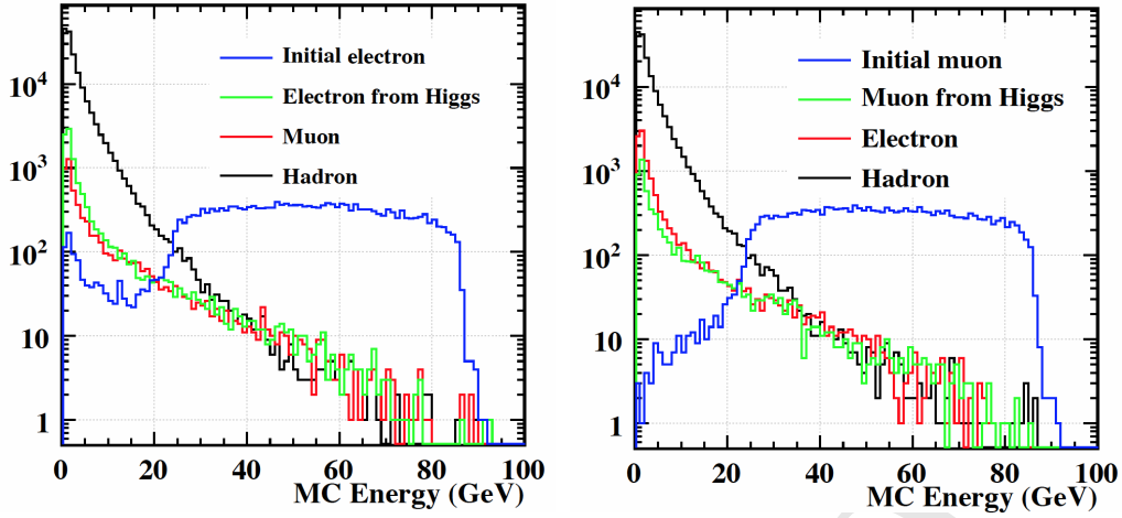
Figure 3.5: Energy spectrum of the leptons and the charged hadrons in the e^+e^-H events (left) and the \mu^+\mu^-H events (right).
