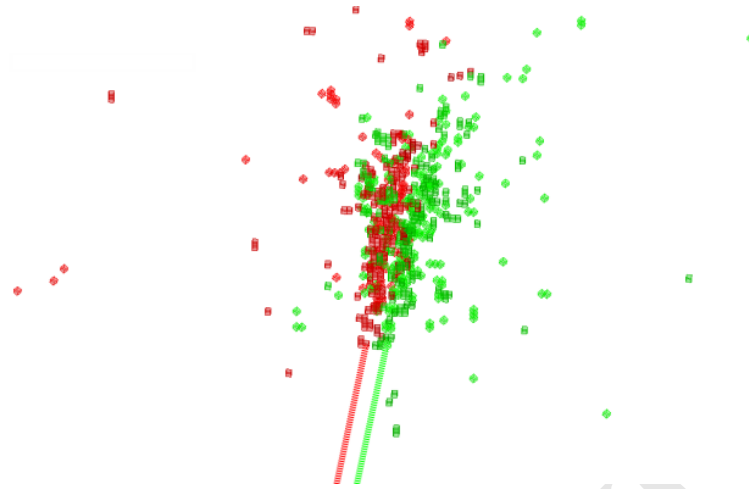
Figure 10.6: A reconstructed di-photon event at Si-W ECAL with 1 mm cell size. Each photon has an energy of 5 GeV, and their impact points are separated by 4 mm.
