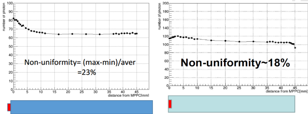
Figure 5.5: Uniformity of scintillator strips with an SiPM coupled on side surface (left) or embedded into one side (right).
