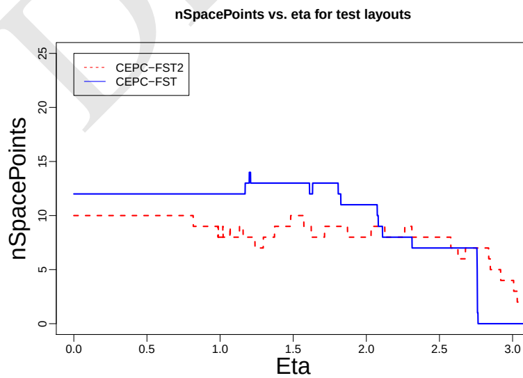
Figure 4.28: The number of expected hits are shown as function of track pseudorapidity.
