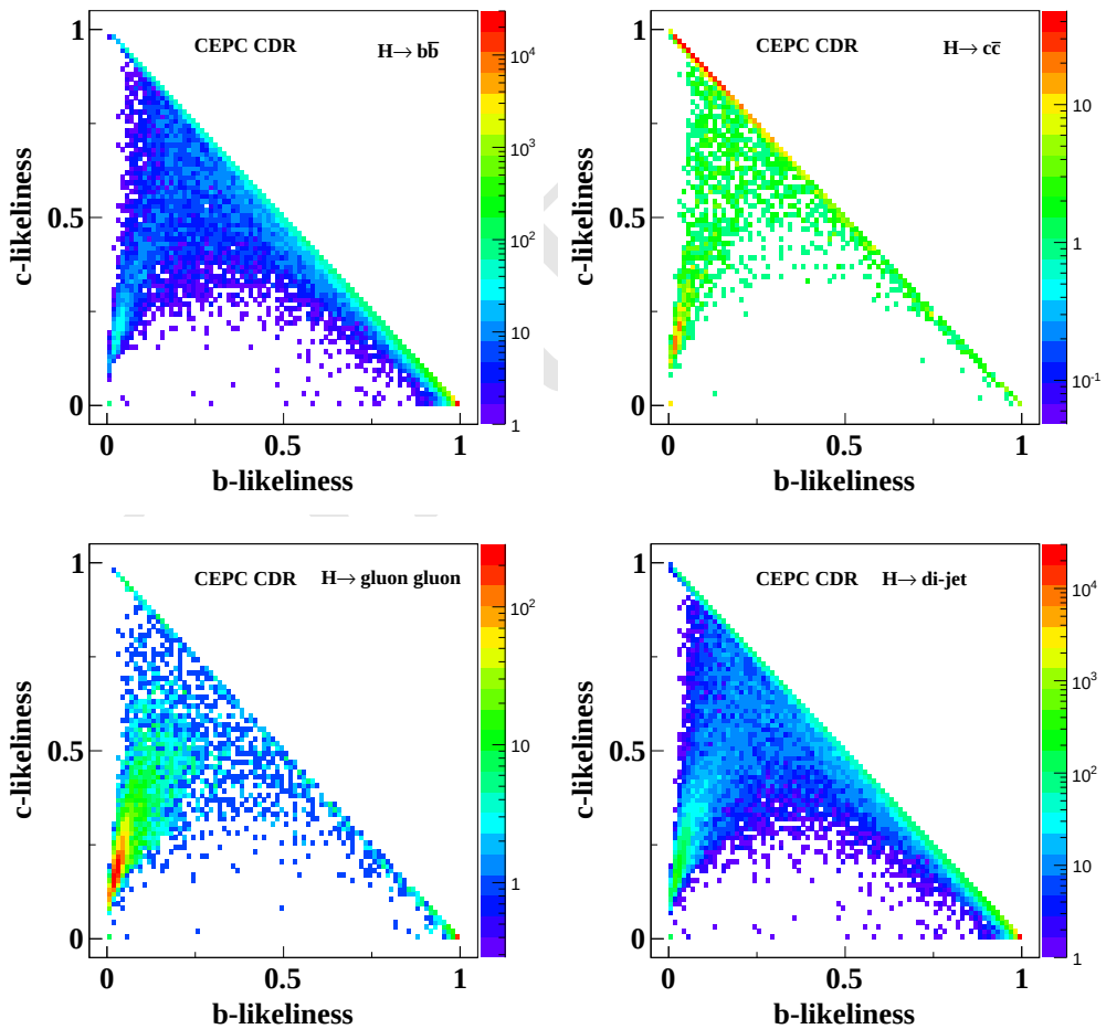
Figure 10.20: The heavy flavor jet likelihoods for Higgs samples: a, H \rightarrow b\bar{b} ; b H \rightarrow c\bar{c} ; c, H \rightarrow gg , and d, H \rightarrow 2\text{jets}
