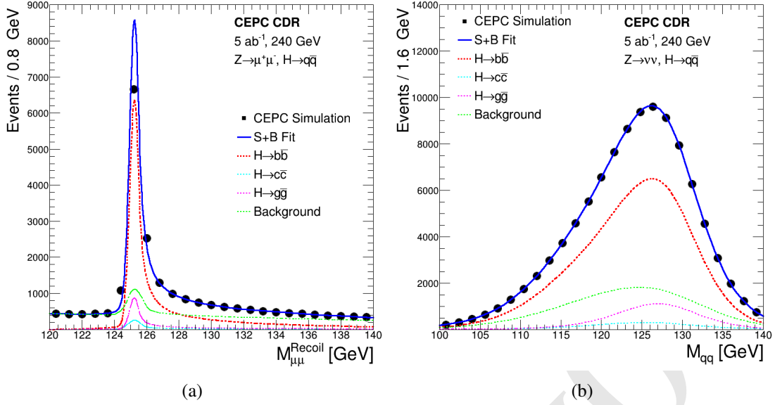
Figure 11.4: (a) e^+e^- \rightarrow ZH production with H \rightarrow b\bar{b}/c\bar{c}/gg : distributions of (a) the recoil mass of Z \rightarrow \mu\mu and (b) the dijet invariant mass distribution for the Z \rightarrow \nu\bar{\nu} decay. Contributions from other Higgs boson decays are included in the background.
