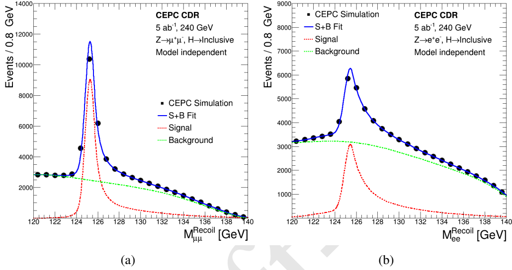
Figure 11.3: The inclusive recoil mass spectra of e^+e^- \rightarrow ZX candidates of (a) Z \rightarrow \mu\mu and (b) Z \rightarrow ee from an integrated luminosity of 5 \text{ ab}^{-1} . No attempt to identify X is made.
