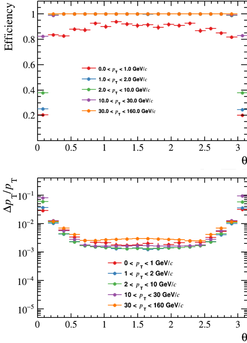
Figure 10.2: Single particle reconstruction efficiency (up plot) and resolution (lower plot) as a function of the track momentum and track polar angle.
