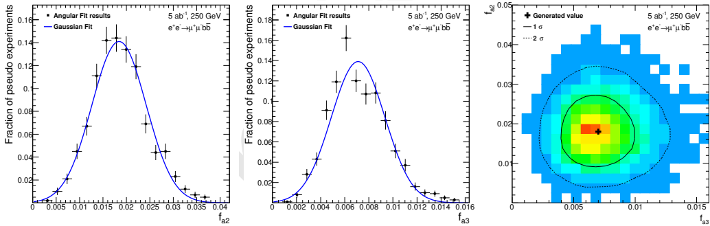
Figure 11.15: Distribution of fitted values of f_{a2} and f_{a3} in a large number of generated experiments. In the left and middle plots, only the parameter shown is floated. Other parameters are fixed to SM expectations. Right plot: simultaneous fit of non-zero f_{a2} and f_{a3} , with 68% and 95% confidence level contours shown.
