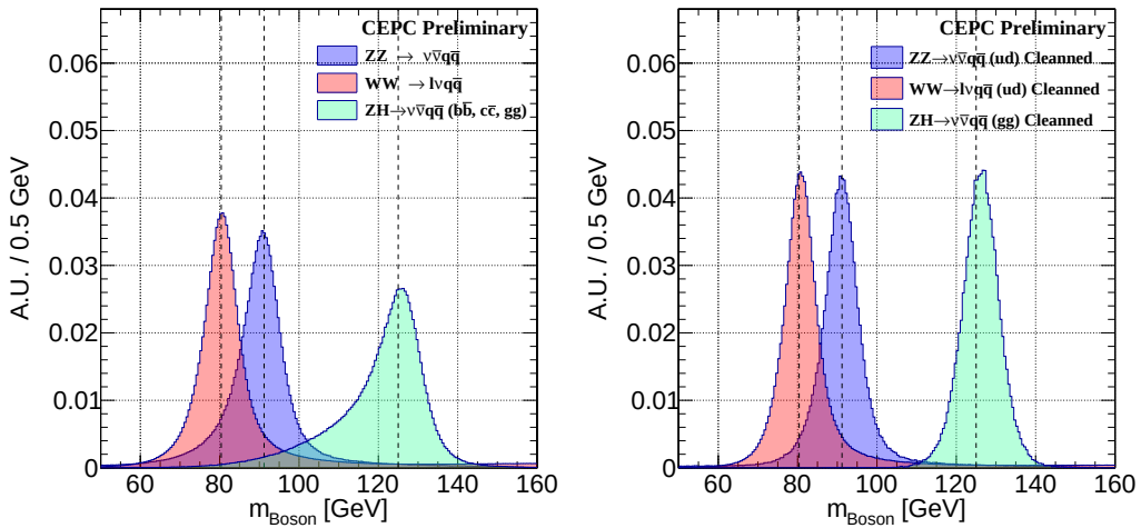
Figure 10.14: Reconstructed boson masses of the inclusive (Left) and cleaned (Right) lvq\bar{q} (red), \nu\tilde{\nu}q\bar{q} (blue) and \nu\tilde{\nu}H, H \rightarrow jj samples (green).
