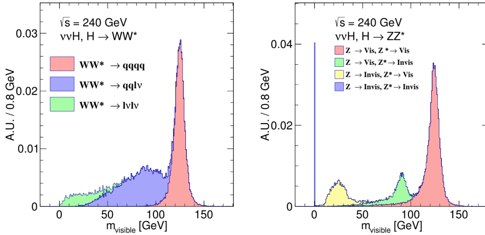
Figure 10.18: Total visible mass distribution of H \rightarrow WW^* (Left) and H \rightarrow ZZ^* events (right).
