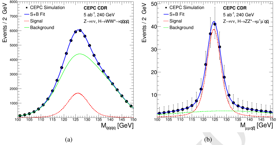
Figure 11.5: (a) e^+e^- \rightarrow ZH production with H \rightarrow WW^* \rightarrow q\bar{q}q\bar{q} and Z \rightarrow \nu\bar{\nu} : the invariant mass distribution of the 4-jet system. (b) e^+e^- \rightarrow ZH production with H \rightarrow ZZ^* \rightarrow \mu^+\mu^-q\bar{q} and Z \rightarrow \nu\bar{\nu} : the invariant mass distribution of the dimuon and dijet system. Contributions from other Higgs boson decays are included in the background.
