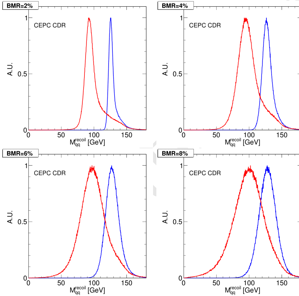
Figure 3.9: Recoil mass distribution of ZZ \rightarrow vvq\bar{q} events and ZH events with Z decays into a pair of quark and Higgs decays invisibly.
