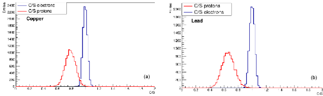
Figure 5.59: C/S ratio (MC simulations) for 80 GeV e^- and protons in (a) copper and (b) lead.
