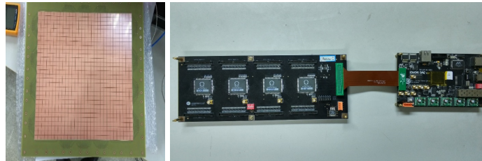
Figure 5.36: Pictures for the phase I design.
