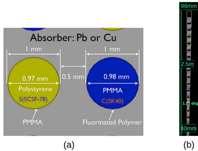
Figure 5.48: (a) Fibre arrangement inside the modules. (b) Dimensions of a module in the barrel region (at \eta = 0 ): from inside to outside the number of fibres more than doubles.
