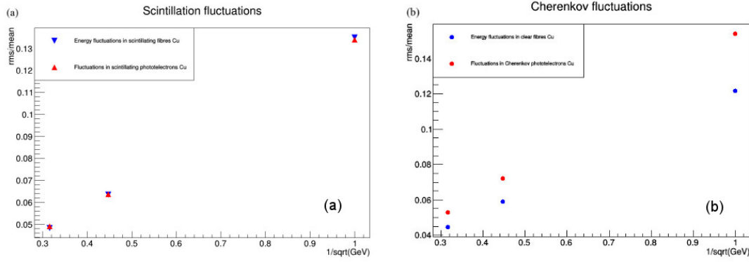
Figure 5.56: Relative fluctuation of the total signal detected in the (a) scintillating and (b) Čerenkov fibres, for both the energy deposit and the number of photoelectrons (MC simulations).
