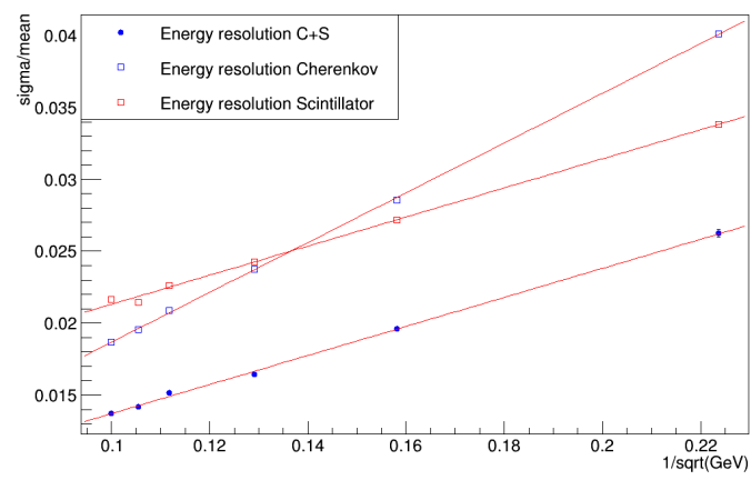
Figure 5.57: Relative resolution for em showers for the C and S signals, independently, and for the average of the two (MC simulations).
