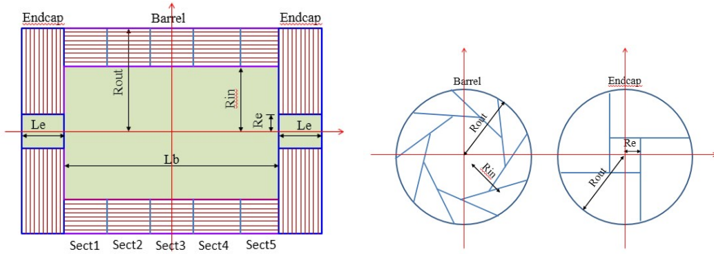
Figure 5.20: HCAL layout in Y-Z plane (left plot), HCAL Barrel layout in X-Y plane (middle plot) and HCAL Endcap layout in X-Y plane (right plot).
