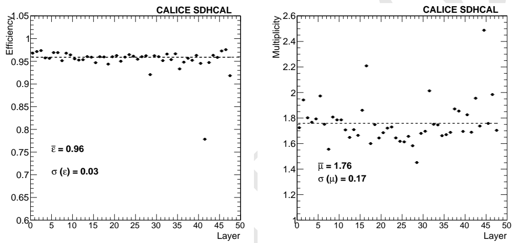
Figure 5.24: Left: Efficiency of the GRPC detectors of the SDHCAL. Right: the pad multiplicity of the GRPCs. One third of the chamber 42 was not instrumented.
