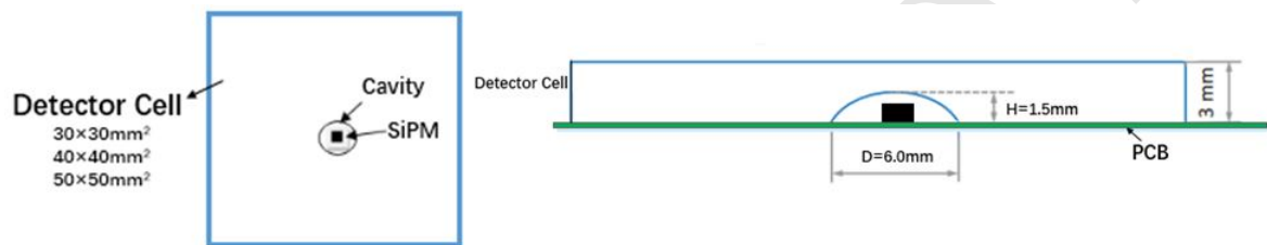
Figure 5.40: Top view of a detector cell (left) and sectional view of a detector cell with a dome-shaped cavity (right)
