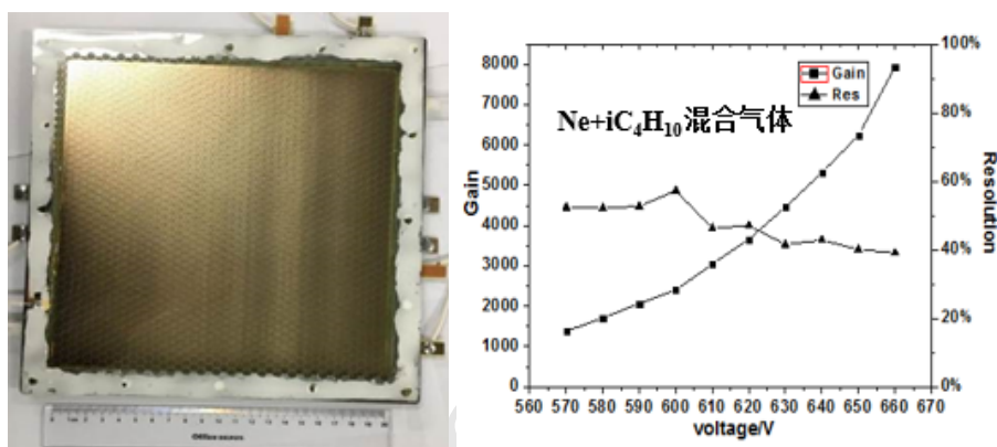
Figure 5.33: The photograph(left) and performance (right) of the WELL-THGEM detector.
