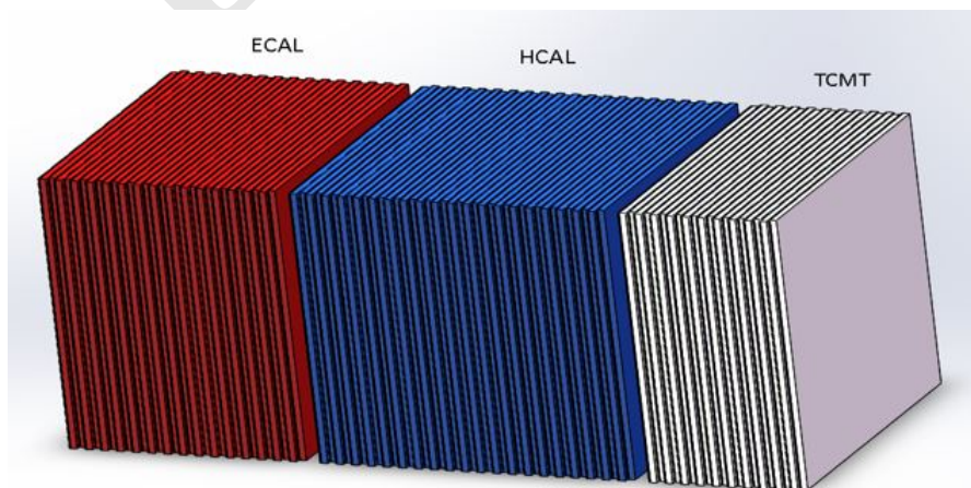
Figure 5.41: The structure of simulated calorimeters which is a part of the simplify geometry. Red part is the the Silicon ECAL, Blue part is the scintillator AHCAL
