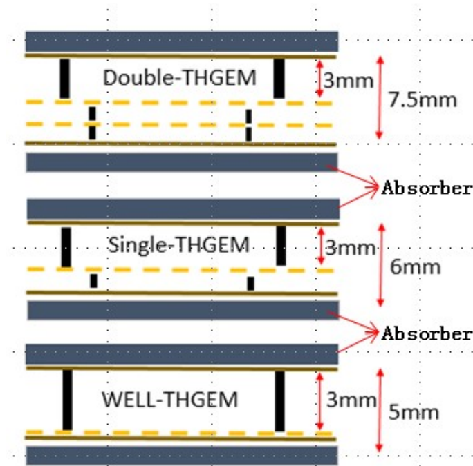
Figure 5.29: Structure of THGEM based detector for DHCAL.
