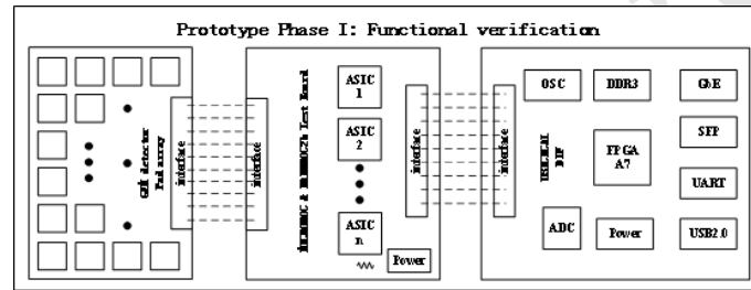
Figure 5.35: The diagram of the phase I design.
