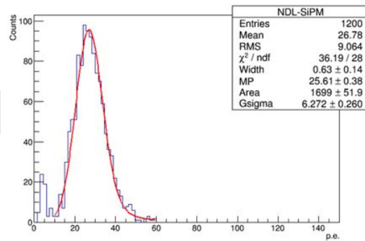
Figure 5.45: Sr-90 electron source test result of scintillator detector cell readout by NDL-SiPM
