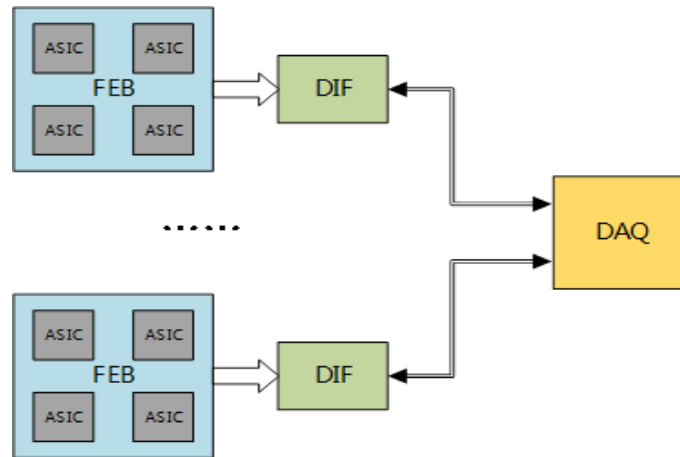
Figure 5.34: The schematic diagram of the readout system.
