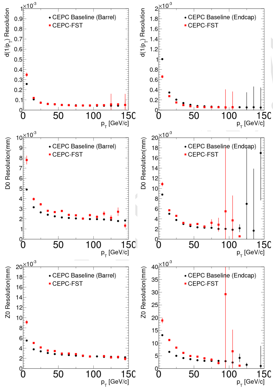
Figure 4.32: The tracking p_T , d0 , and z0 resolutions are measured as function of p_T , \phi , and \theta using single muons, left in the barrel region and right in the endcap region. They are compared between CEPC v_4 and CEPC-FST detectors.
