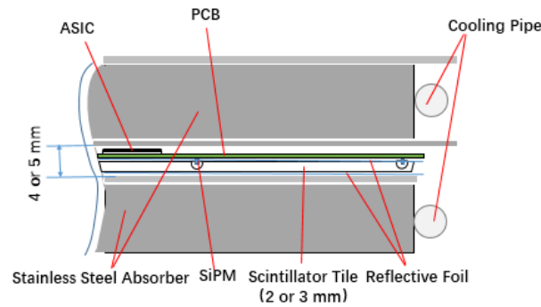
Figure 5.39: Side view of one layer in AHCAL
