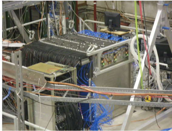
Figure 5.23: The SDHCAL prototype in beam test at CERN.
