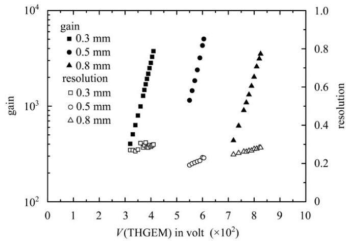
Figure 5.30: Gain and energy resolution of THGEM detector obtained with ^{55}\text{Fe} .
