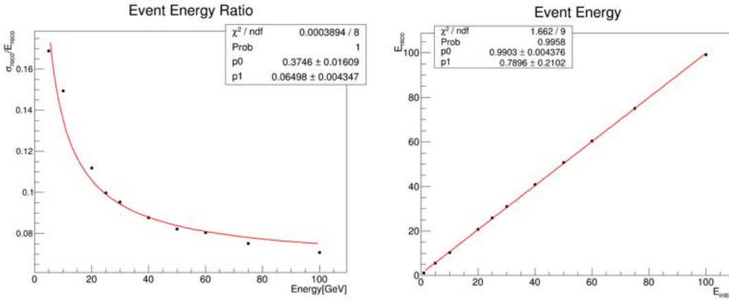
Figure 5.42: Left figure is energy resolution, right figure is the result of reconstruction energy linearity
