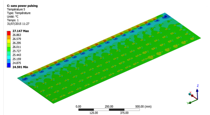
Figure 5.28: Temperature distribution in an active layer of the SDHCAL operated with no power-pulsing. The cooling system is made of a circulating water inside copper tubes in contact with the ASICs.
