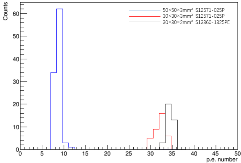
Figure 5.43: The uniformity measurement result of 30 \times 30 \times 3 \text{ mm}^3 , 50 \times 50 \times 3 \text{ mm}^3 and 30 \times 30 \times 2 \text{ mm}^3 detector cell
