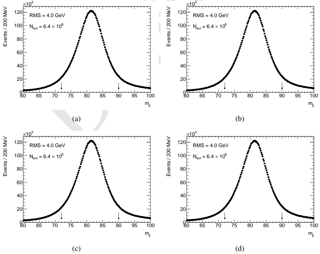
Figure 11.18: Dijet invariant mass distributions for WW \rightarrow \mu\nu qq events, without (a) and with (b) a b -jet veto cut, and for ZZ \rightarrow \mu\mu qq events, without (c) and with (d) a b -jet veto cut. The numbers of events and RMS of the distributions are quoted for the interval indicated by the arrows.
