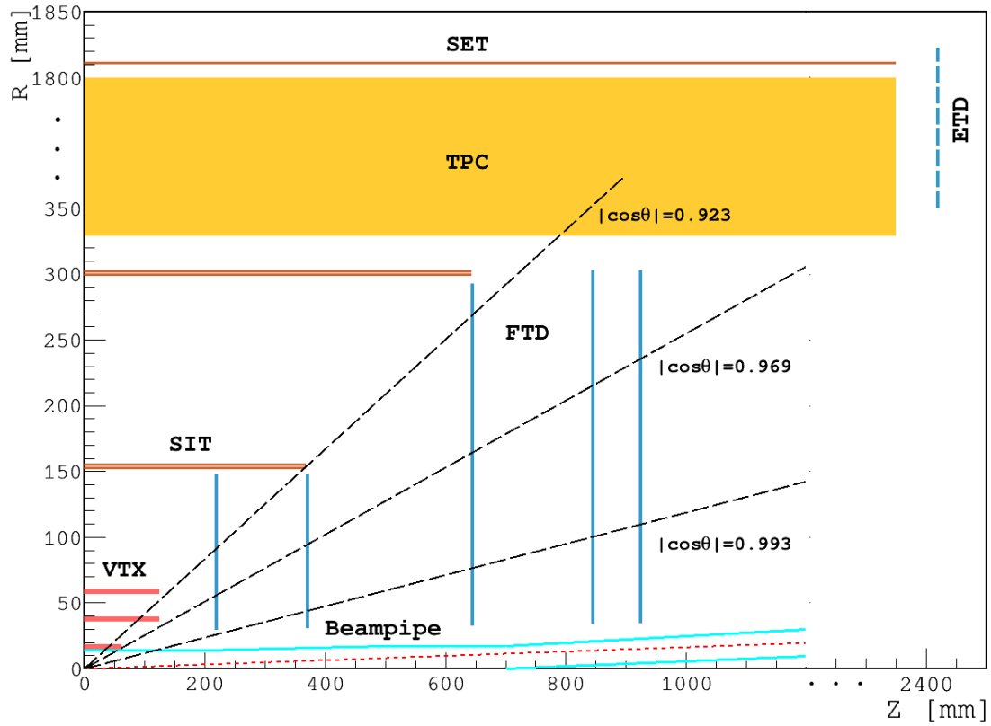
Figure 4.22: Preliminary layout of the CEPC silicon tracker. The red lines indicate positions of the vertex detector layers, orange lines for the SIT and SET components of the silicon tracker, the gray-blue lines for the FTD and ETD components of the silicon tracker, and the cyan lines for the beampipe. The ETD line is a dashed line because it is not in the present full simulation.
