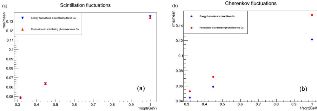
Figure 5.46: Relative fluctuation of the total signal detected in the (a) scintillating and (b) Čerenkov fibers, for both the energy deposit and the number of photoelectrons (MC simulations).
