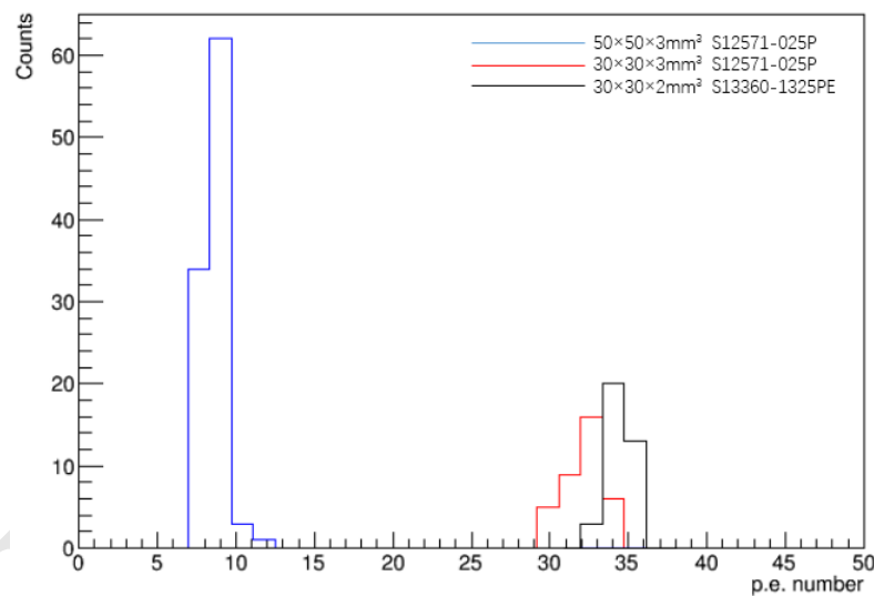
Figure 5.34: The uniformity measurement result of 30\times30\times3\text{mm}^3 (red histogram, p.e. is about 30-34), 50\times50\times3\text{mm}^3 (blue histogram, p.e. is about 8-10) and 30\times30\times2\text{mm}^3 (black histogram, p.e. is about 34-36) detector cell.
