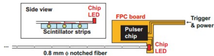
Figure 5.16: Schematic of the SiPM gain monitoring system with LED and notched fibre. Light pulses from the LED are scattered and distributed into each strip.
