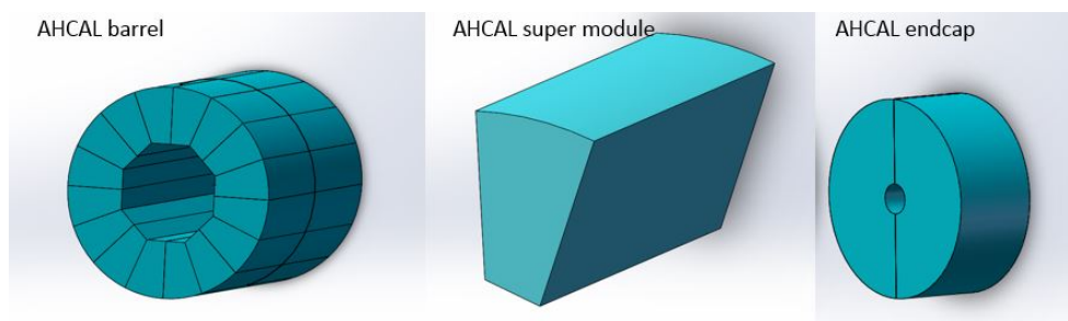
Figure 5.29: The layout of AHCAL barrel (left plot) and endcap regions (right plot), the middle plot shows a super module of AHCAL. The total thickness of AHCAL is about 100cm. The AHCAL barrel consists of 32 super modules, each with 40 layers.
