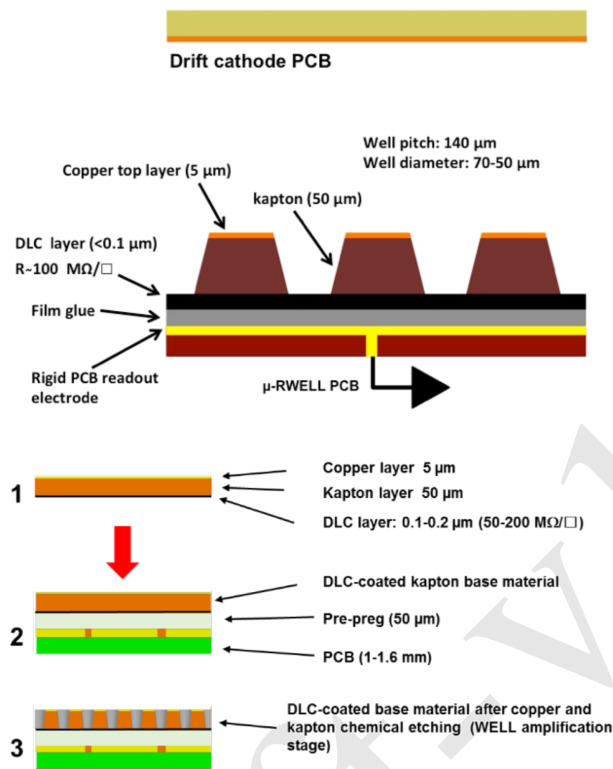
Figure 7.2: a) Layout of a \mu -RWELL detector module with the cathode and the \mu -RWELL PCBs; b) Coupling steps of the \mu -RWELL PCB.
