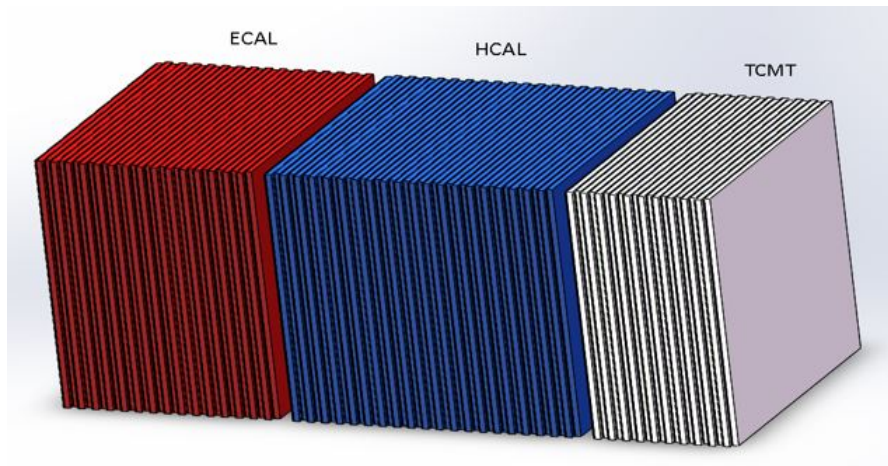
Figure 5.32: The structure of simulated calorimeters which is a part of the simplified geometry. Red part is the Silicon ECAL (30-layer), Blue part is the scintillator AHCAL (40-layer), Grey part is the tail catcher (20-layer).
