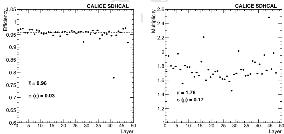
Figure 5.21: Left: Efficiency of the GRPC detectors of the SDHCAL, the average efficiency is 0.96 \pm 0.03 . Right: The pad multiplicity of the GRPCs, it is 1.76 \pm 0.17 . (Note: Figures taken from [14].)
