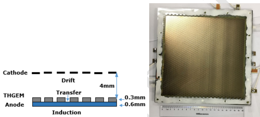
Figure 5.28: The schematic diagram of the WELL-THGEM (left plot), the thickness is 5mm. A 20\text{cm} \times 20\text{cm} WELL-THGEM detector was produced (right plot).
