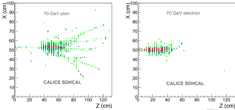
Figure 5.22: Left: Event display of an 70 GeV pion interaction in the SDHCAL prototype. Right: Event display of a 70 GeV electron interaction in the SDHCAL prototype. (Note: Figures taken from [14].)
