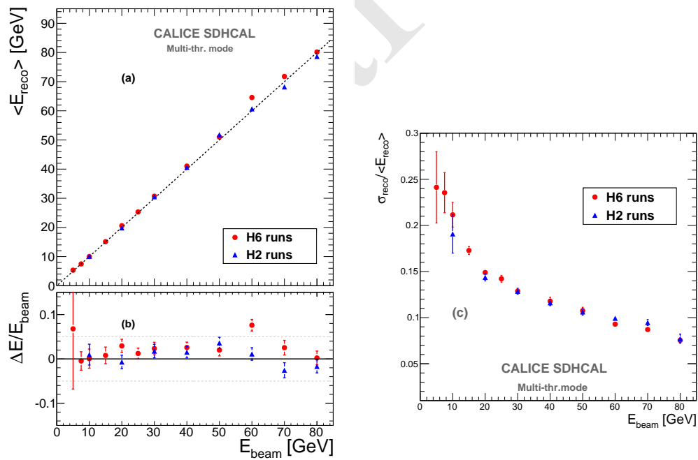
Figure 5.23: Left: a) Reconstructed energy of the hadronic showers collected in both H2 and H6 SPS beamlines. b) The relative deviation of the reconstructed energy with respect to the beam energy. Right: Relative energy resolution of the reconstructed hadronic shower. The pion beam of H6 beamline is largely contaminated by protons at high energy (>50 GeV). (Note: Figures taken from [14].)
