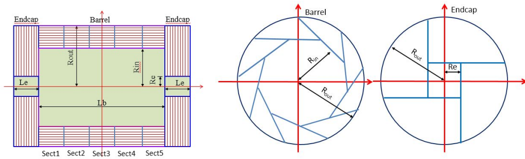
Figure 5.17: HCAL layout in Y-Z plane (left plot), HCAL Barrel layout in X-Y plane (middle plot) and HCAL Endcap layout in X-Y plane (right plot). The inner radius in X-Y plane is 2300mm, the outer radius is 3340mm. The inner and outer of HCAL endcap in Z-axis are 2670mm and 3710mm, respectively.
