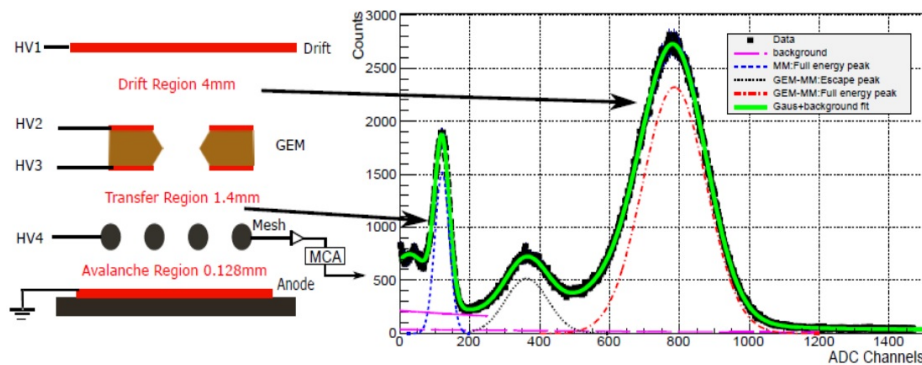
Figure 4.17: Energy spectrum of the hybrid structure TPC detector module with 55 Fe radioactive source. (The green curve is the whole energy spectrum from the hybrid detector, the last two peaks amplified by GEM and Micromegas, the first two peaks amplified by Micromegas only.)
