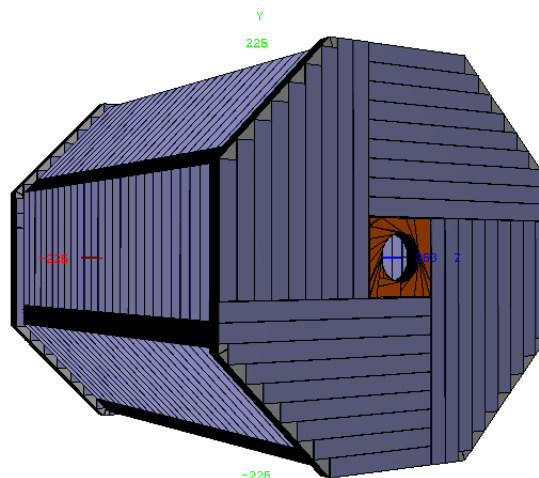
Figure 5.6: Schematic of the CEPC ECAL layout in its baseline design. The ECAL is organized into one cylindrical barrel and two disk-like end-cap sections, with 30 layers in each section. The barrel section is arranged into 8 staves, each consisting of 5 trapezoidal modules. Each of the two endcap sections is made of four quadrants, each consisting of 2 modules. The ECAL barrel overall radius is 2028mm in X-Y plane, the two end-caps are located at \pm 2635 mm.
