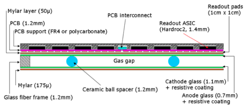
Figure 5.19: Cross-sectional view of an active layer with GRPC and readout layer. The GRPC gas gap is 1.2mm, with two glass plates of 1.1mm (cathode plate) and 0.7mm (anode plate) thickness. The thickness of PCB is 1.2mm and that of readout ASIC is 1.4mm.
