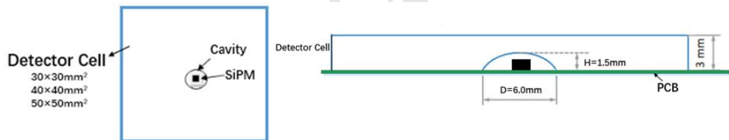
Figure 5.31: Top view of a detector cell (left plot) and cross-sectional view of a detector cell with a dome-shaped cavity (right plot). The detector cell size varies from 30 \times 30mm^2 , 40 \times 40mm^2 to 50 \times 50mm^2 . The height of dome-shaped cavity in the center of detector cell is 1.5mm with diameter of 6mm.
