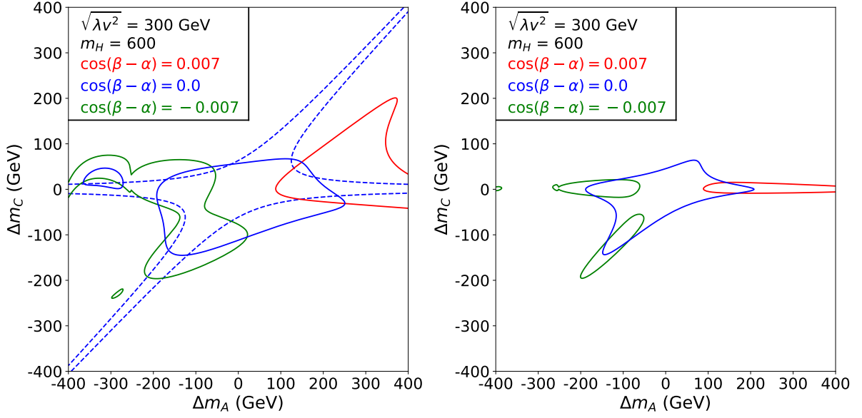
Figure 2.37: Allowed regions of \Delta m_A = m_A - m_H and \Delta m_C = m_{H^\pm} - m_H at 95% C.L., for different choices of \cos(\beta - \alpha) . Left: Higgs precision constraints for \cos(\beta - \alpha) = 0.007 (solid red), 0 (solid blue), and -0.007 (solid green) and Z -pole constraints (dashed blue). Note that the Z -pole constraints are the same for \cos(\beta - \alpha) = 0.007, 0, and -0.007 . Right: constraints from combining both the Higgs and Z pole measurements for \cos(\beta - \alpha) = 0.007 (solid red), 0 (solid blue), and -0.007 (solid green). Plots are taken from Ref. [380]. Add GeV to m_H = 600 .
