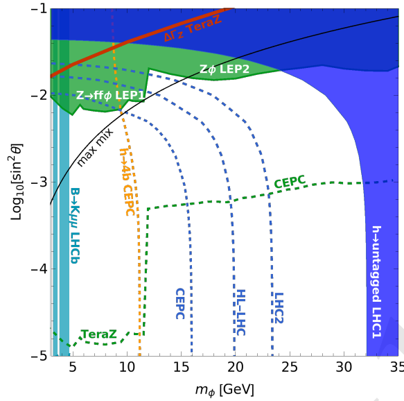
Figure 2.9: Constraints on the relaxion mass m_\phi and relaxion-Higgs mixing angle \sin^2 \theta from the non-Standard Model decay of the Higgs into relaxion pairs, adapted from [35]. Shaded regions indicate current exclusions from LEP and the LHC. Dashed blue lines indicate the reach of CEPC and future operation of the LHC in searches for untagged non-Standard Model decays of the Higgs, while the orange dashed line indicates the reach of CEPC in searches for h \rightarrow \phi\phi \rightarrow 4b . The green dashed line indicates the reach of CEPC's Z -pole run in searches for e^+e^- \rightarrow Z\phi .
