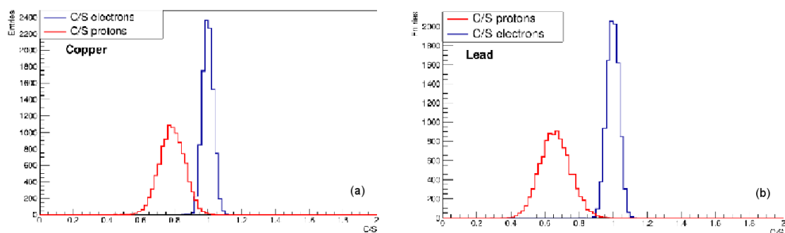
Figure 5.49: C/S ratio (MC simulations) for 80 GeV e^- and protons in (a) copper and (b) lead.
