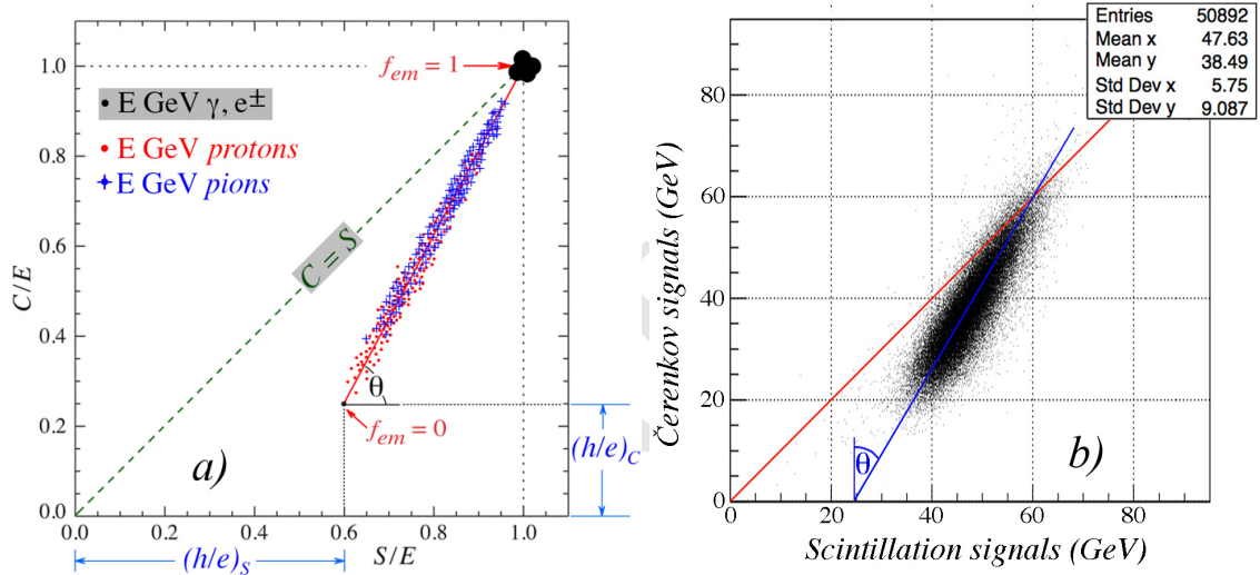
Figure 5.36: (a) Scatter plot of C/E versus S/E in a dual-readout calorimeter for p and \pi ; (b) scatter plot of C and S signals for 60 GeV pions in the RD52 lead-fiber calorimeter.
