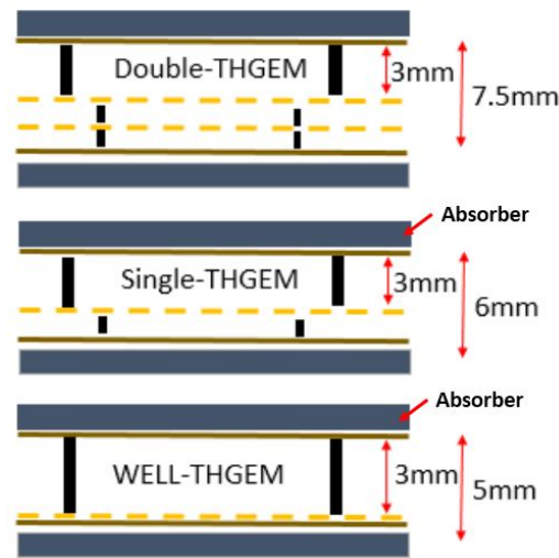
Figure 5.25: Schematic of three different types of THGEMs, eg. doubly-THGEM with thickness of 7.5mm (top plot), single-THGEM with thickness of 6mm (middle plot) and well-THGEM with thickness of 5mm (bottom plot).
