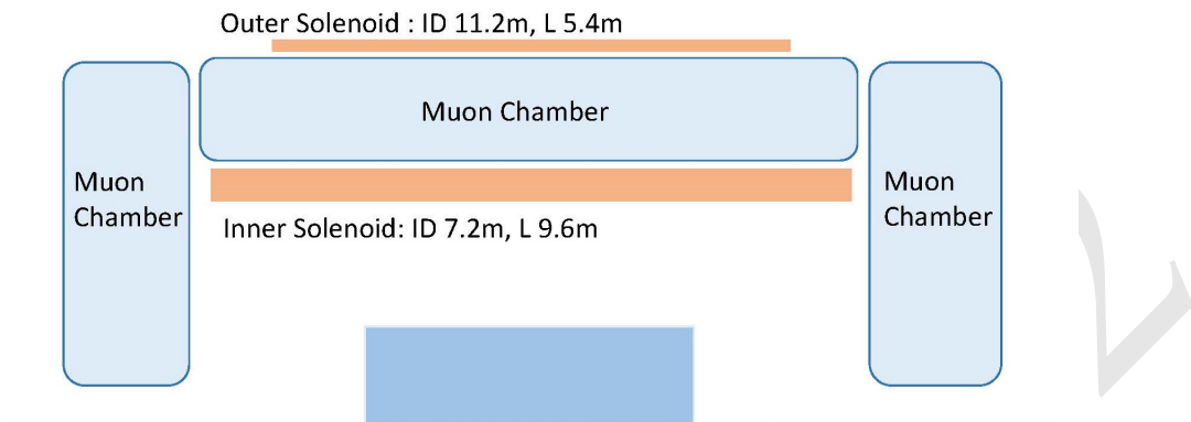
Figure 6.5: The sketch of dual solenoid design. The main solenoid provides central field within the room temperature bore. The outer solenoid provides the stray field shielding and a magnetic field between the two solenoids to facilitate muon tracking. The inner diameter of the main solenoid is 7.2 m. The inner diameter of the outer solenoid is 11.2 m.
