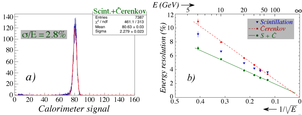
Figure 5.43: In the RD52 copper-fiber module: (a) signal distribution of the sum of all fibers for 40 GeV electrons; (b) the em energy resolution as a function of the beam energy. Shown are the results for the two types of fibers, and for the average combined signal.
