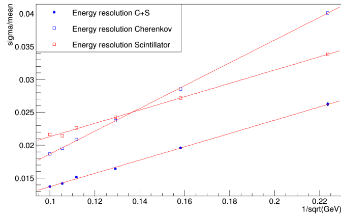
Figure 5.47: Relative resolution for em showers for the C and S signals, independently, and for the average of the two (MC simulations).
