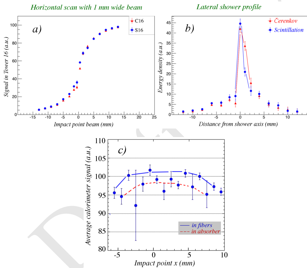
Figure 5.42: (a) The signal from a 1 mm wide beam of 100 GeV electrons, in the RD52 lead-fiber prototype, as a function of the impact point; (b) the lateral shower profiles derived from this measurement; (c) the dependence of the scintillation signal on impact point for a beam impinging parallel to the fibers.
