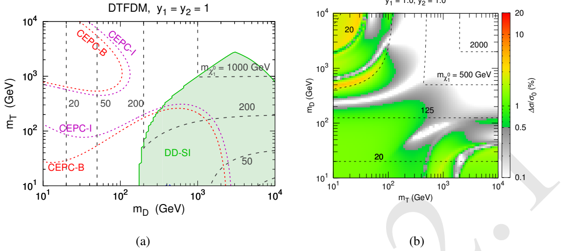
Figure 2.21: (a) The CEPC electroweak precision ( S, T ) fit probe of the doublet–triplet model at the custodially symmetric point y_1 = y_2 = 1 , taken directly from Figure 5a of Ref. [150]. When the dark matter particle is mostly triplet ( m_D \gg m_T ), spin-independent direct detection is a powerful probe (shaded green region). When the dark matter particle is mostly doublet, the tree-level direct detection rate vanishes but CEPC’s measurement of the S parameter becomes a powerful probe (dashed contours). (b) CEPC’s sensitivity to the same model via the Higgsstrahlung cross section \sigma(ZH) , taken directly from Figure 11b of Ref. [153]. We see that in a large part of parameter space with m_T \gg m_D , where the direct detection rate is low due to custodial symmetry, there are observable (percent-level or higher) deviations in the ZH cross section.
