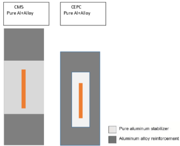
Figure 6.4: The baseline design for the CEPC solenoid conductor. The conductor is wrapped around purity aluminium stabilizer and aluminium alloy reinforcement with coextrusion technology. The Rutherford cable contains 32 NbTi strands. The overall dimensions of this conductor are 22 mm × 56 mm.
