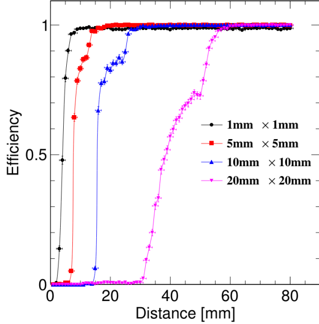
Figure 5.5: Reconstruction efficiency of events with two parallel 5 GeV photons as a function of the distance between the two photons for different ECAL sensor sizes. The reconstruction of the di-photon events is fully efficient once the sensor size is smaller than half of the distance between the two photons.
