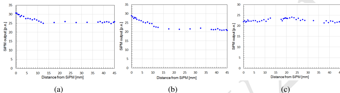
Figure 5.11: Light output of a scintillator sensitive unit with three SiPM coupling configurations: side (a), bottom-end (b), bottom-center (c). The bottom-center configuration gives the best uniformity of 10% without reduction of light output.
