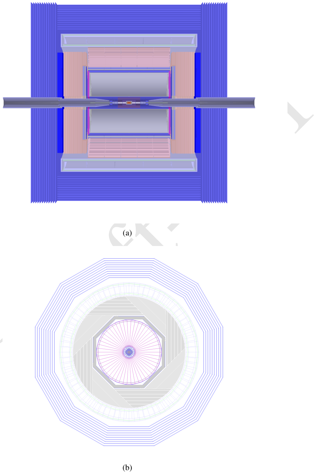
Figure 3.9: The RZ (a) and R- \phi (b) view of the baseline detector concept. The baseline concept uses a double beam with 33 mrad crossing angle, and has a short L^* of 2.2 meter. In the central Barrel, from inner to outer, the baseline concept is composed of a Vertex system, a Silicon Inner Tracker, a TPC, a Silicon External Tracker, an ECAL, an HCAL, a Solenoid of 3 Tesla and a Return Yoke. In the forward region, 5 pairs of tracking disks are installed to enlarge the tracker acceptance (from |\cos(\theta)| < 0.99 to |\cos(\theta)| < 0.996 ).
