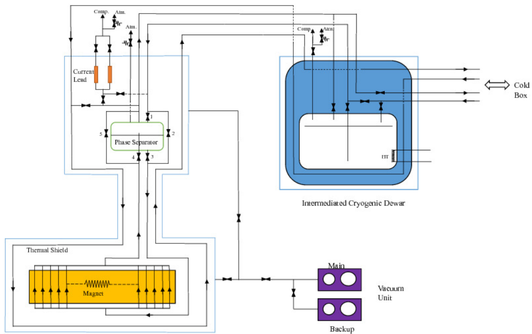
Figure 6.5: The thermosiphon cooling circuit of the superconducting coil.
