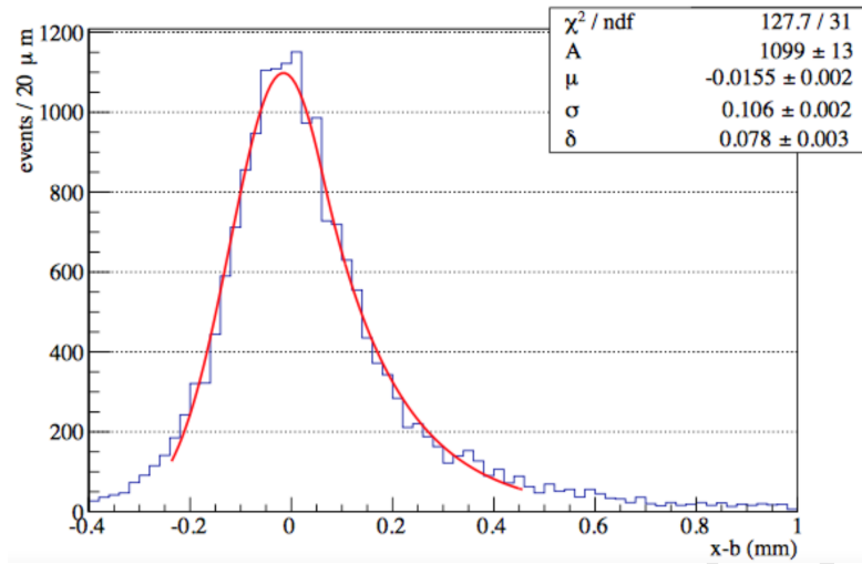
Figure 4.31: Measured drift distance residual distribution in the MEG2 drift chamber prototype using a 85%He-15% i\text{C}_4\text{H}_{10} gas mixture. Cosmic rays tracks indicate a resolution better than 110 \mu\text{m} , averaged over all drift times and in a wide range of track angles.
