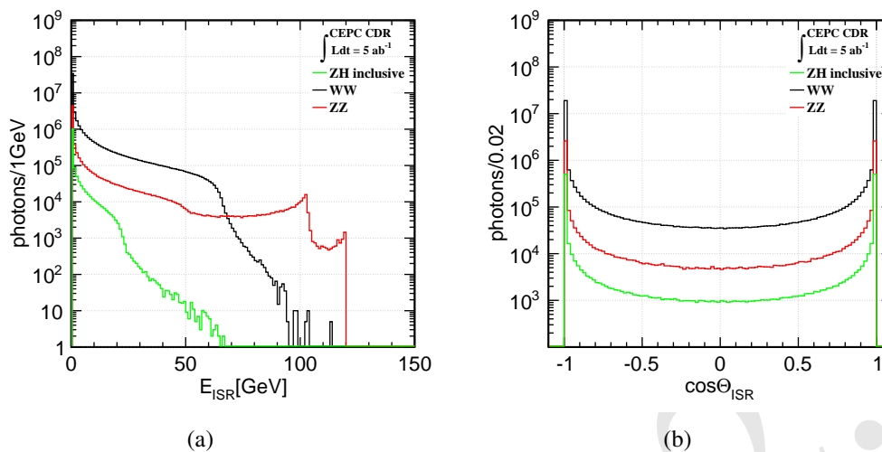
Figure 3.6: The energy and polar angle distributions of ISR photons from WW , ZZ , and ZH events at the CEPC Higgs operation, normalized to 5 \text{ ab}^{-1} integrated luminosity. These ISR photons are concentrated at forward region (see the right hand plot).
