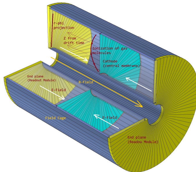
Figure 4.6: Sketch of the TPC detector structure. The TPC is a cylindrical gas detector with an axial electric field formed between the end-planes (yellow) and a central cathode plane/membrane (light blue). The cylindrical walls of the volume form the electric field cage (dark blue). Charged particles passing through the chamber are bent by the axial magnetic field and gas ionization electrons drift to the end plates where they are collected by readout modules (yellow).
