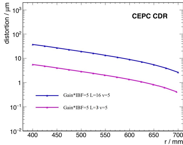
Figure 4.14: Distortion as a function of the electron initial radial position r for different parameters: Gain for the GEM-MicroMegas hybrid, IBF is the ions backflow reducing rate, L is the luminosity, and v is the drift velocity of the ions in m/s.
