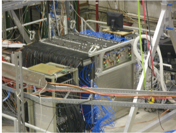
Figure 5.20: The SDHCAL prototype in beam test at CERN.
