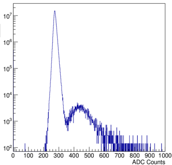
Figure 5.14: The pulse height distribution for cosmic-ray signals of the scintillator sensitive unit with a 10 μm SiPM. Cosmic-ray signals can be found well separated from noise demonstrating the sensitivity of the scintillator sensitive unit to M.I.Ps.
