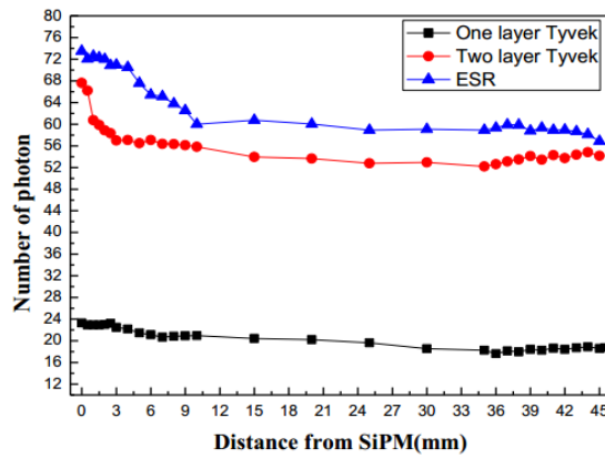
Figure 5.12: Light yields of scintillator strips with different reflectors versus the distance of an incident particle from SiPM . The scintillator with ESR gives the highest light yield.
