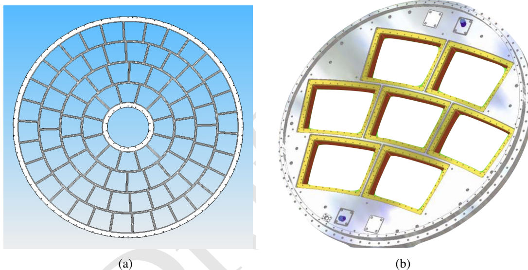
Figure 4.7: Mechanical support (TPC endwall) for mounting the readout modules. Each opening will take a readout module of roughly 170 mm \times 210 mm. (a) Full size design of TPC endwall; (b) Small prototype of the endwall showing details of the openings for the module insertion. The readout modules will be inserted, and installed on the inside of the endwall to minimize dead space.
