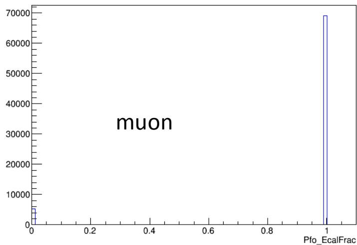
EcalFrac: e_{\text{cale}} / (e_{\text{cale}} + h_{\text{cale}})
