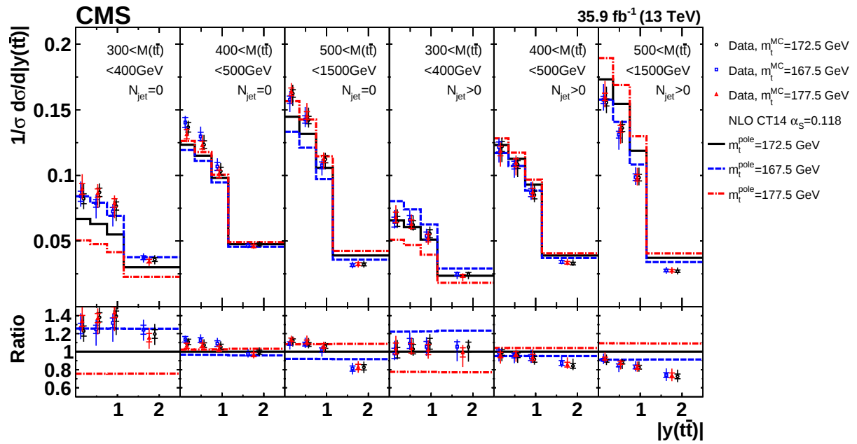
Figure C.1: Comparison of the measured [N_{\text{jet}}^{0,1+}, M(\bar{t}t), y(\bar{t}t)] cross sections obtained using different values of m_t^{\text{MC}} to NLO predictions obtained using different m_t^{\text{pole}} values (further details can be found in Fig. 3).
