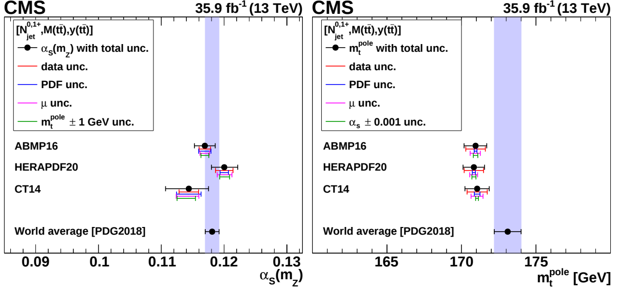
Figure 18: The \alpha_s(m_Z) (left) and m_t^{pole} (right) values extracted at NLO using different PDFs. The contributions to the total uncertainty arising from the data, PDF, scale, and \alpha_s(m_Z) uncertainties are shown separately. The world average values \alpha_s(m_Z) = 0.1181 \pm 0.0011 and m_t^{pole} = 173.1 \pm 0.9 GeV from Ref. [94] are shown for reference.
