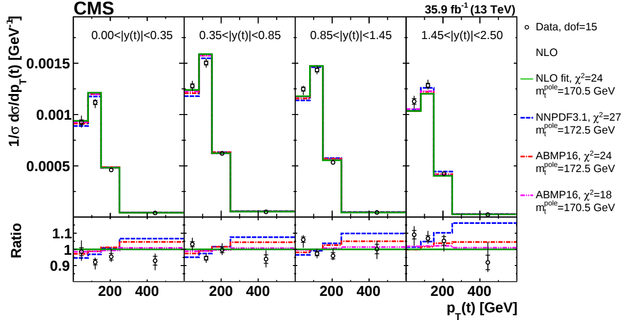
Figure 20: Comparison of the measured [y(t), p_T(t)] cross sections to the NLO predictions using the parameter values from the simultaneous PDF, \alpha_S and m_t^{\text{pole}} fit of the [N_{\text{jet}}^{0,1+}, M(t\bar{t}), y(t\bar{t})] cross sections, as well as the predictions obtained using the NNPDF3.1 and ABMP16 PDF sets with different values of m_t^{\text{pole}} (see Fig. 3 for further details). In the lower panel, the ratios of the data and theoretical predictions to the predictions from the fit are shown. For each theoretical prediction, values of \chi^2 and dof for the comparison to the data are reported.
