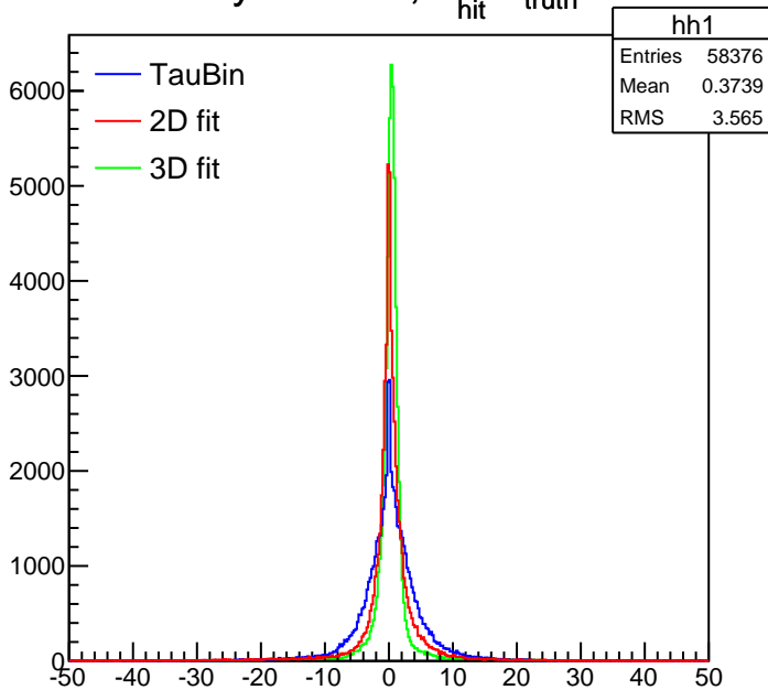
layer:21-24, Z_{\text{hit}} - Z_{\text{truth}}
