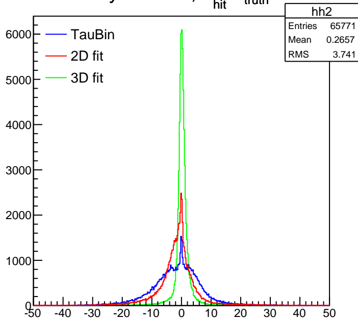
layer:25-28, Z_{\text{hit}} - Z_{\text{truth}}
