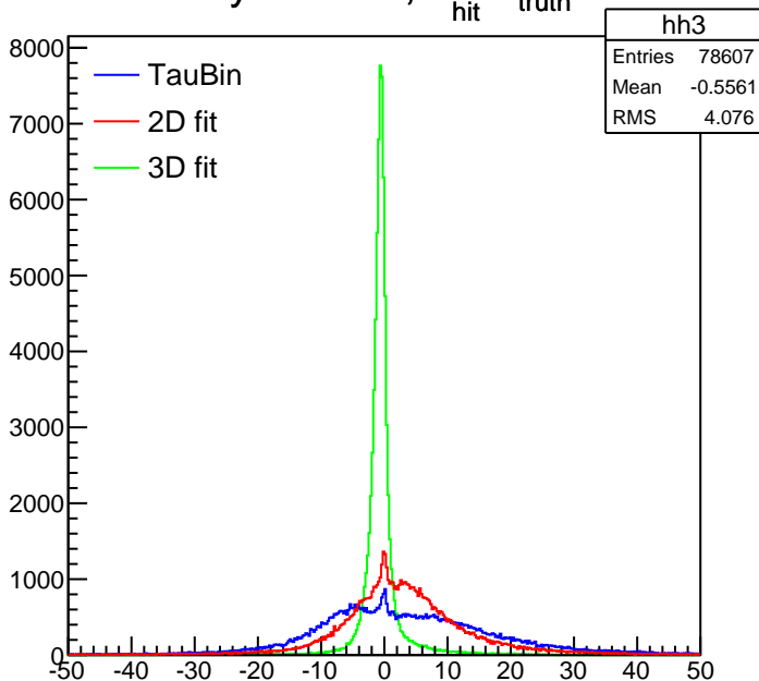
layer:29-32, Z_{\text{hit}} - Z_{\text{truth}}
