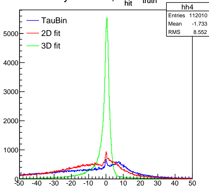
layer:33-36, Z_{\text{hit}} - Z_{\text{truth}}
